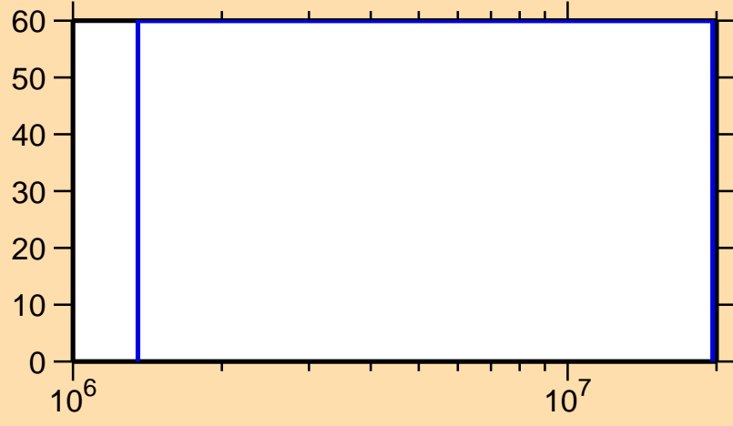
\Delta\sigma/\sigma vs. E for ^{246}\text{Am}(n,n\text{cont.})
