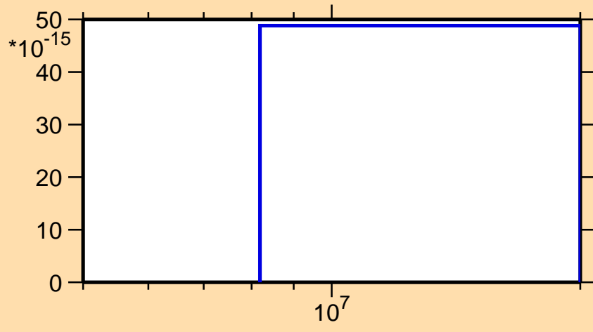
\sigma vs. E for ^{246}\text{Am}(n,3n\alpha)
