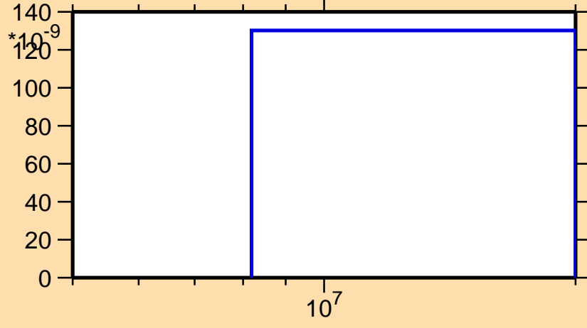
\sigma vs. E for ^{246}\text{Am}(n,nd)
