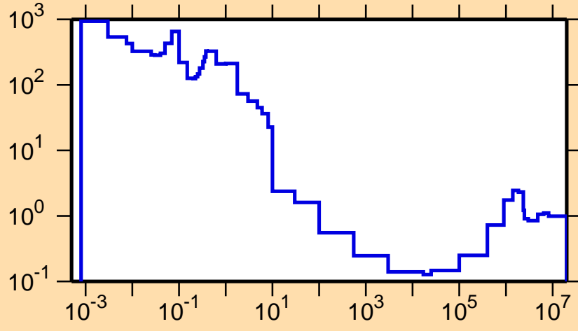
\sigma vs. E for ^{246}\text{Am}(n,f)
