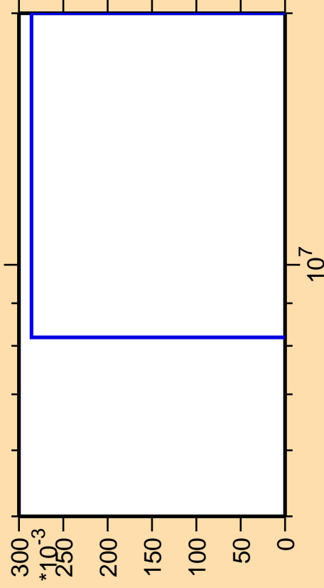
\Delta\sigma/\sigma vs. E for ^{246}\text{Am}(n,3n\alpha)
