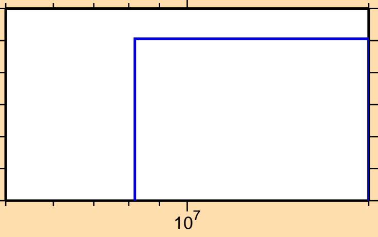
\sigma vs. E for ^{246}\text{Am}(n,nt)
