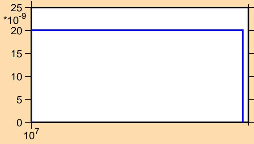
\sigma vs. E for ^{247}\text{Am}(n,\text{nd})
