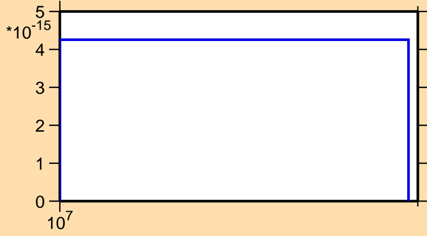
\sigma vs. E for ^{247}\text{Am}(n,\text{He}3)
