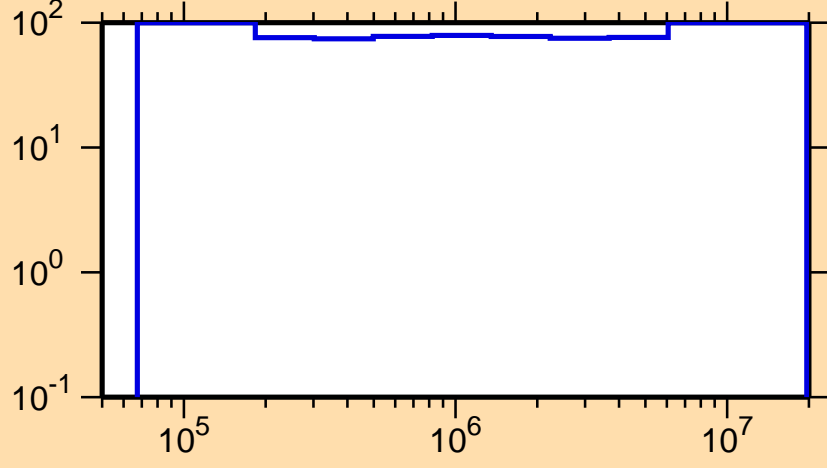
\Delta\sigma/\sigma vs. E for ^{247}\text{Am}(n,\text{inel.})
