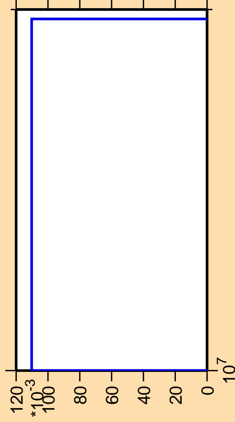
\Delta\sigma/\sigma vs. E for ^{247}\text{Am}(n,3n\alpha)
