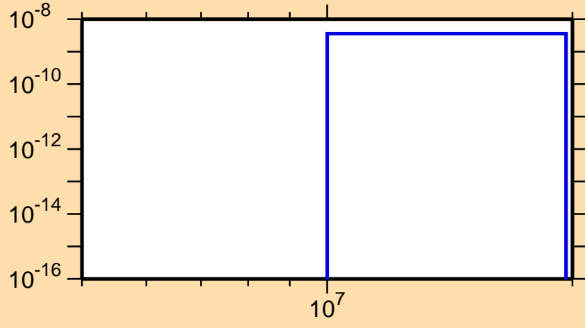
\sigma vs. E for ^{247}\text{Am}(n,2n\alpha)
