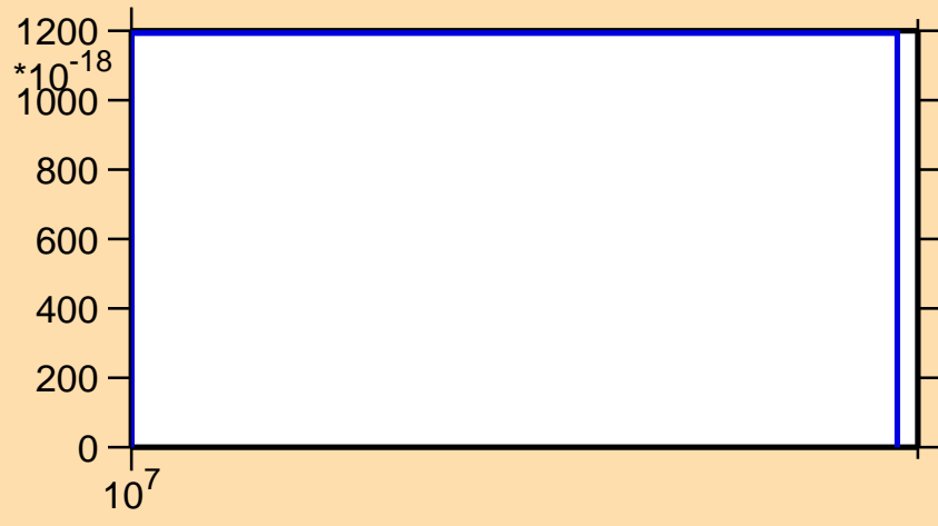
\sigma vs. E for ^{247}\text{Am} (mt 42)
