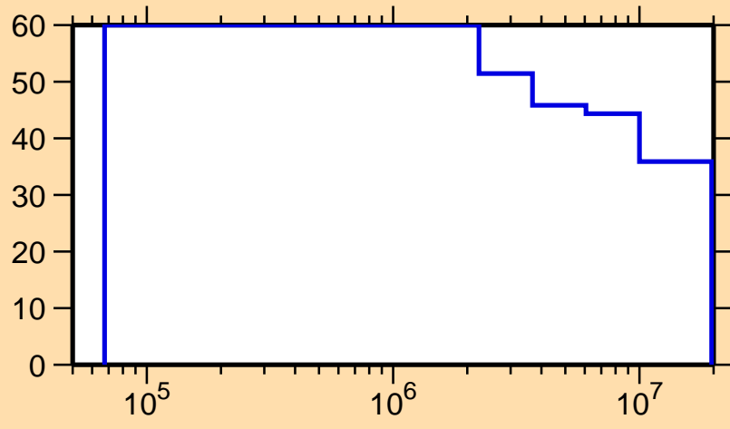
\Delta\sigma/\sigma vs. E for ^{247}\text{Am}(n,\text{nonel.})
