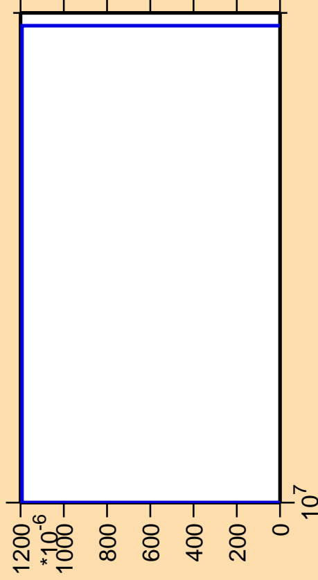
\Delta\sigma/\sigma vs. E for ^{247}\text{Am} (mt 42)
