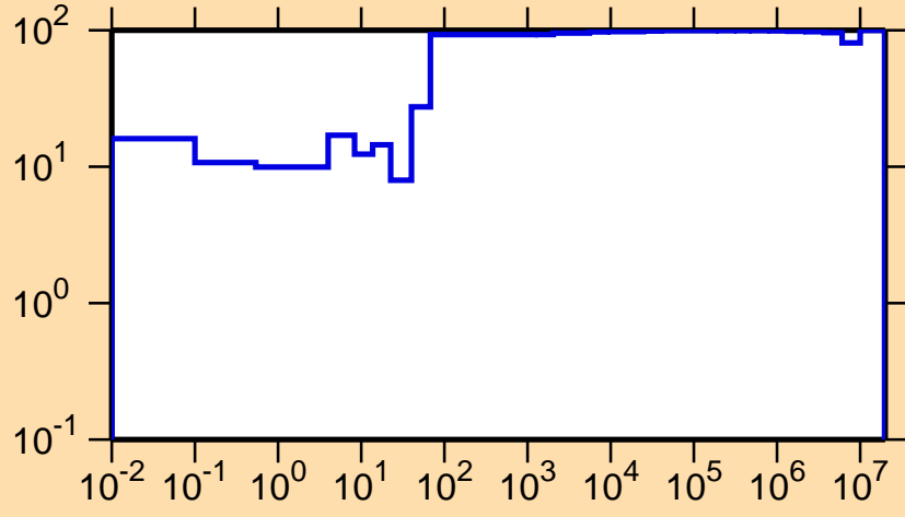
\Delta\sigma/\sigma vs. E for ^{247}\text{Am}(n,\gamma)
