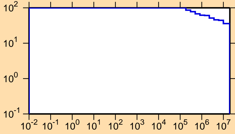
\Delta\sigma/\sigma vs. E for ^{247}\text{Am}(n,\text{nonel.})
