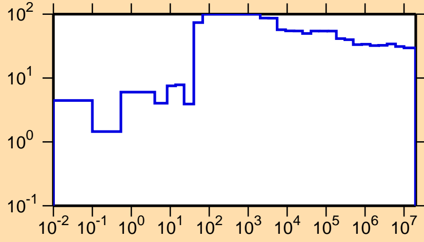
\Delta\sigma/\sigma vs. E for ^{247}\text{Am}(n,\text{tot.})
