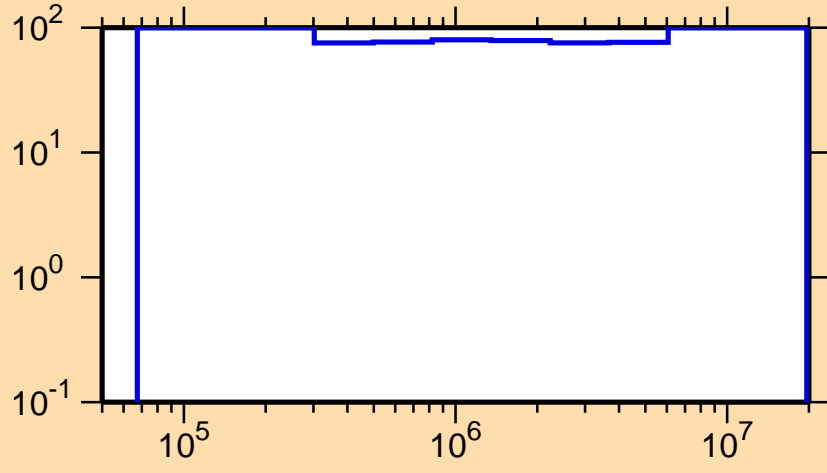
\Delta\sigma/\sigma vs. E for ^{247}\text{Am}(n,n\text{cont.})
