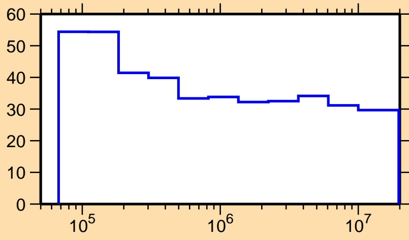
\Delta\sigma/\sigma vs. E for ^{247}\text{Am}(n,\text{tot.})
