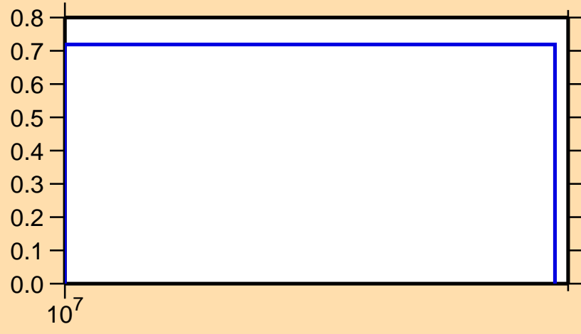
\sigma vs. E for ^{247}\text{Am}(n,3n)
