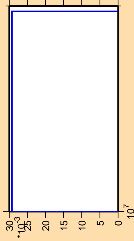
\Delta\sigma/\sigma vs. E for ^{247}\text{Am}(n,\text{He}3)
