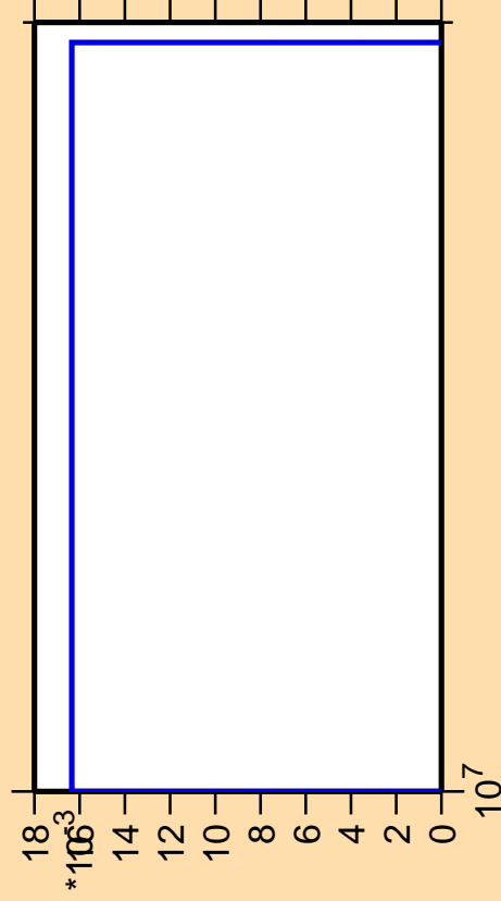
\Delta\sigma/\sigma vs. E for ^{247}\text{Am} (mt 11)
