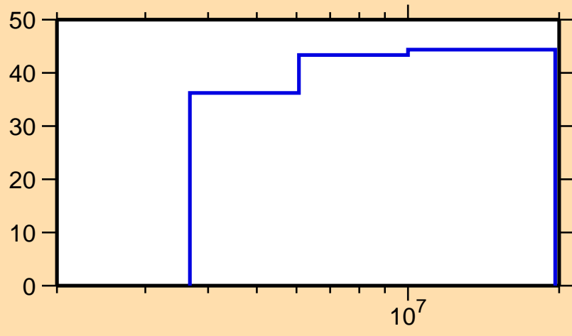
\Delta\sigma/\sigma vs. E for ^{247}\text{Am}(n,\text{el.})
