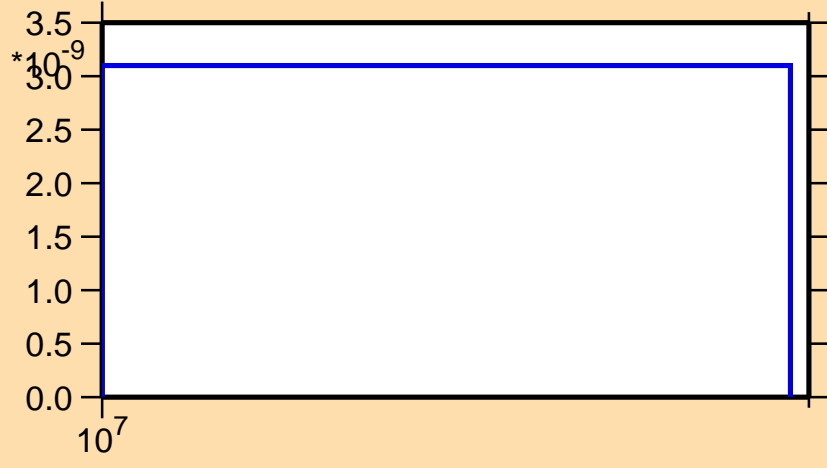
\sigma vs. E for ^{247}\text{Am}(n,2np)
