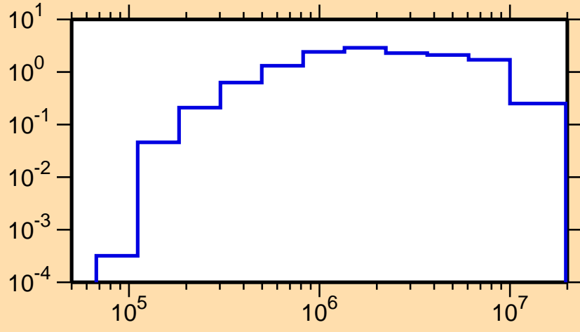
\sigma vs. E for ^{247}\text{Am}(n,n\text{cont.})
