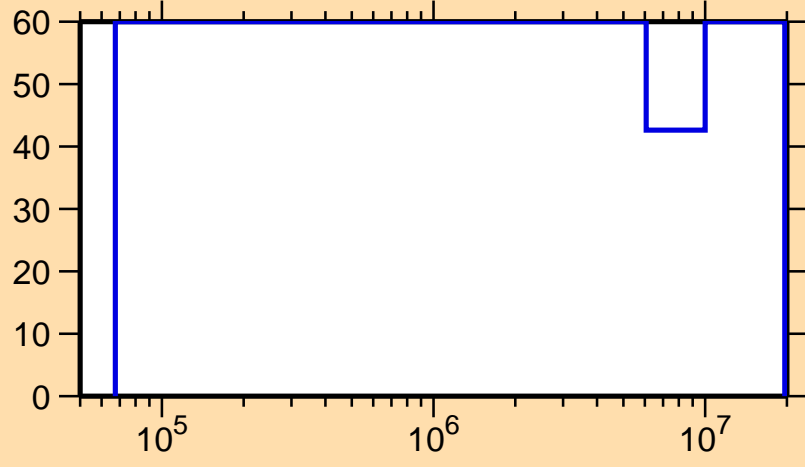
\Delta\sigma/\sigma vs. E for ^{247}\text{Am}(n,n_1)
