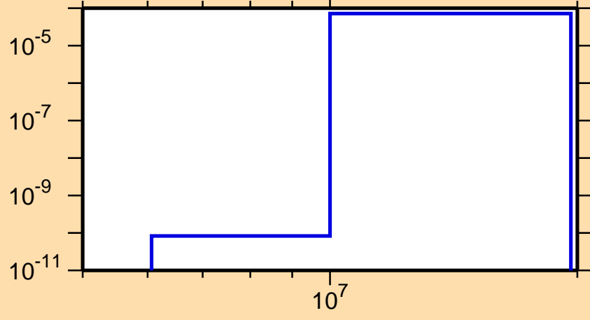
\sigma vs. E for ^{247}\text{Am}(n,d)
