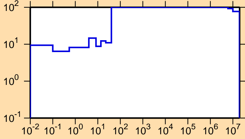
\Delta\sigma/\sigma vs. E for ^{247}\text{Am}(n,f)
