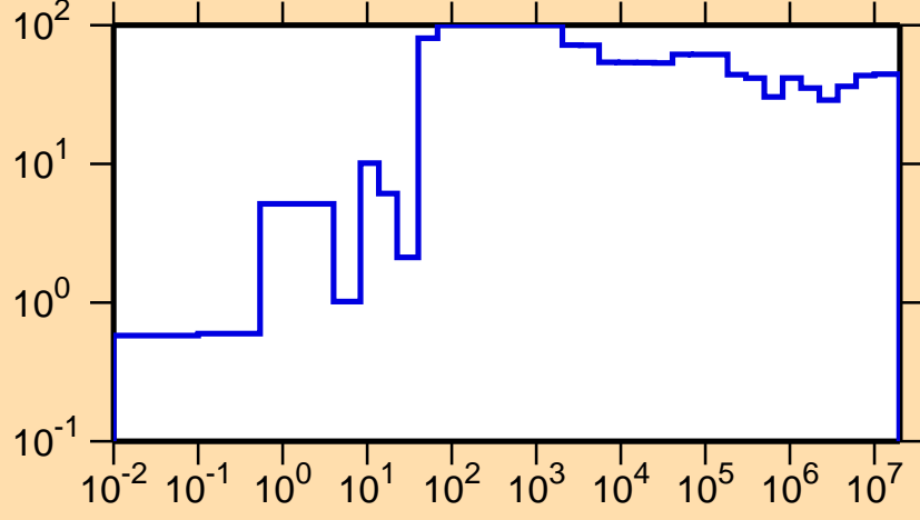
\Delta\sigma/\sigma vs. E for ^{247}\text{Am}(n,\text{el.})
