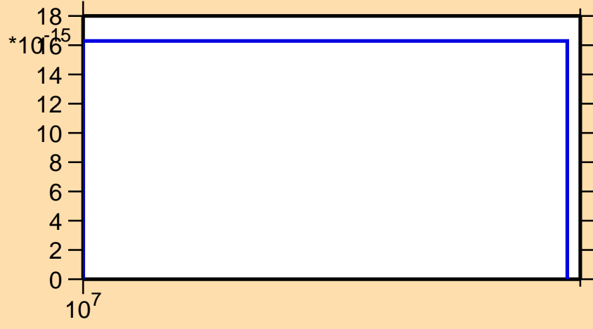
\sigma vs. E for ^{247}\text{Am} (mt 11)
