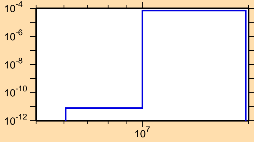
\sigma vs. E for ^{247}\text{Am}(n,np)
