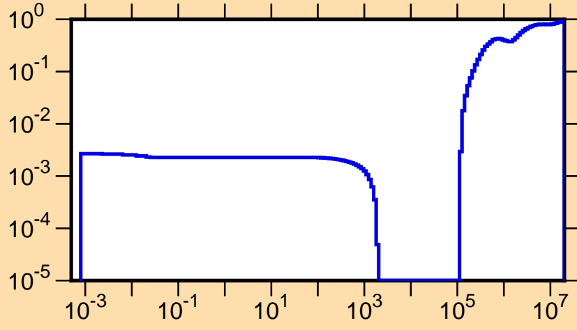
\mu vs. E for ^{248}\text{Am}(\text{mt251})
