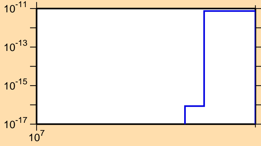
\sigma vs. E for ^{248}\text{Am} (mt 11)
