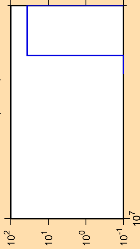
\Delta\sigma/\sigma vs. E for ^{248}\text{Am} (mt 11)
