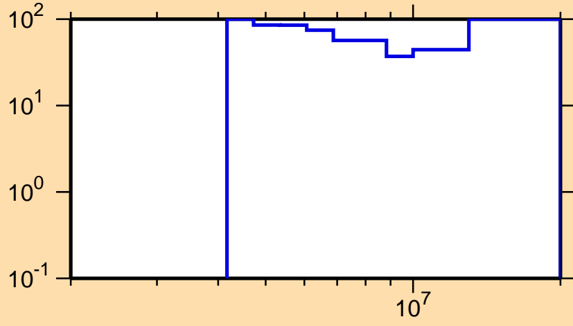
\Delta\sigma/\sigma vs. E for ^{248}\text{Am}(n,2n)
