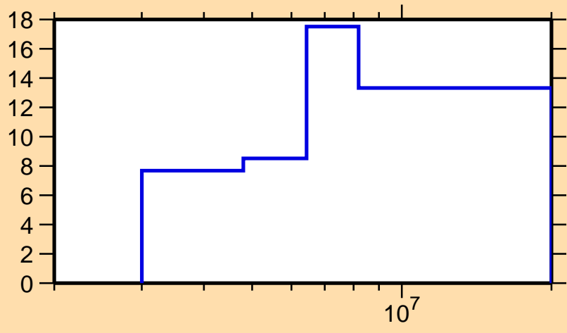
\Delta\sigma/\sigma vs. E for ^{248}\text{Am}(n,\text{tot.})
