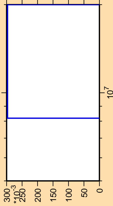
\Delta\sigma/\sigma vs. E for ^{248}\text{Am}(\text{mt } 11)
