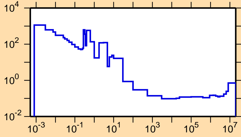
\sigma vs. E for ^{248}\text{Am}(n,f)
