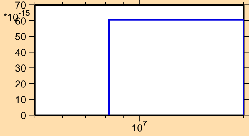
\sigma vs. E for ^{248}\text{Am}(\text{mt } 11)
