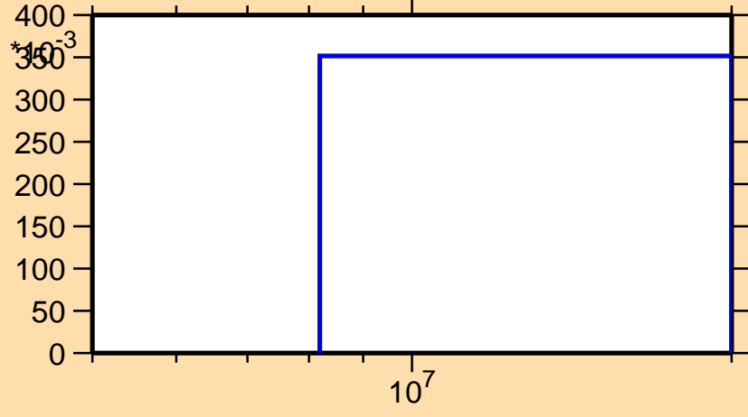
\sigma vs. E for ^{248}\text{Am}(n,3n)
