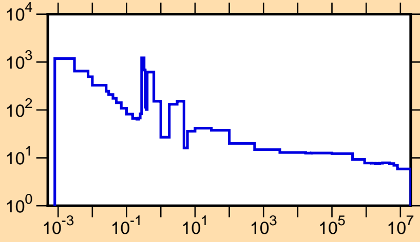
\sigma vs. E for ^{248}\text{Am}(n,\text{tot.})
