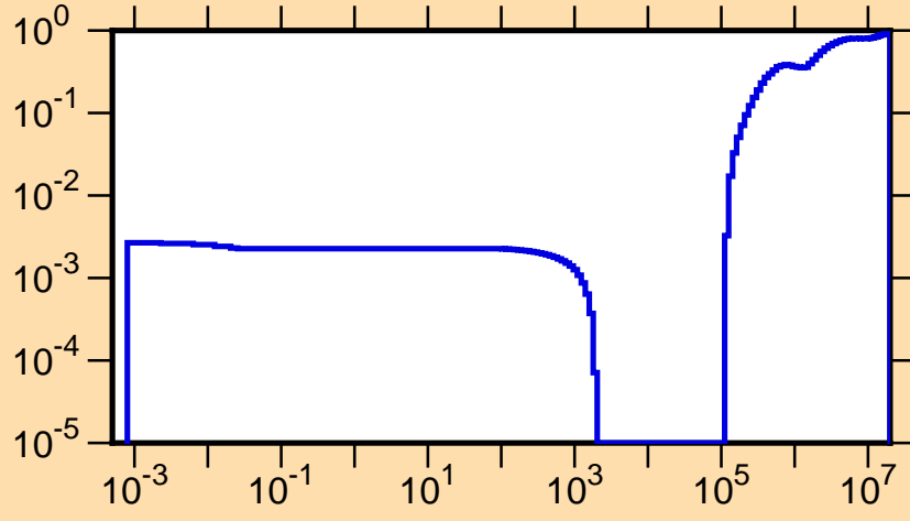
\mu vs. E for ^{249}\text{Am}(\text{mt251})
