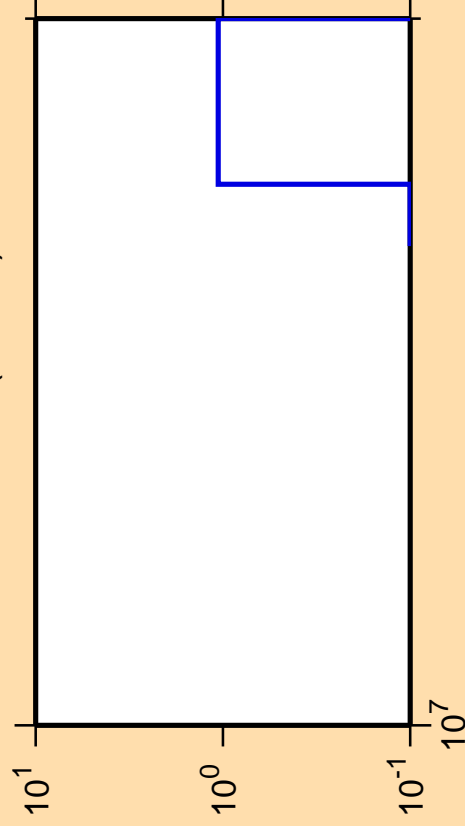
\Delta\sigma/\sigma vs. E for ^{249}\text{Am}(n,\text{He3})
