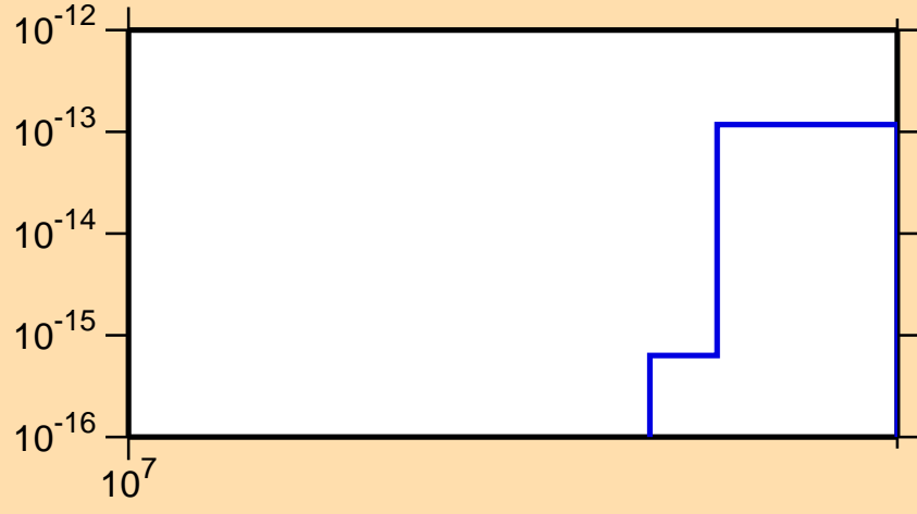
\sigma vs. E for ^{249}\text{Am}(n,\text{He3})
