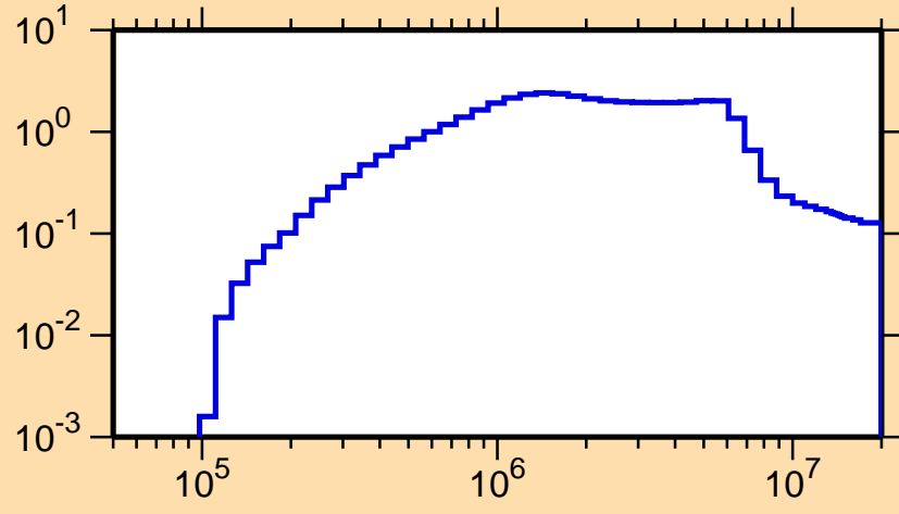
\sigma vs. E for ^{249}\text{Am}(n,n\text{cont.})
