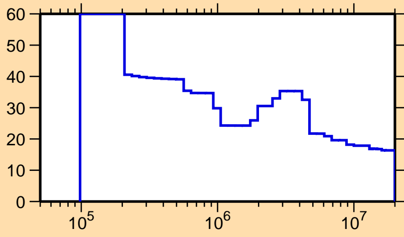
\Delta\sigma/\sigma vs. E for ^{249}\text{Am}(n,\text{nonel.})
