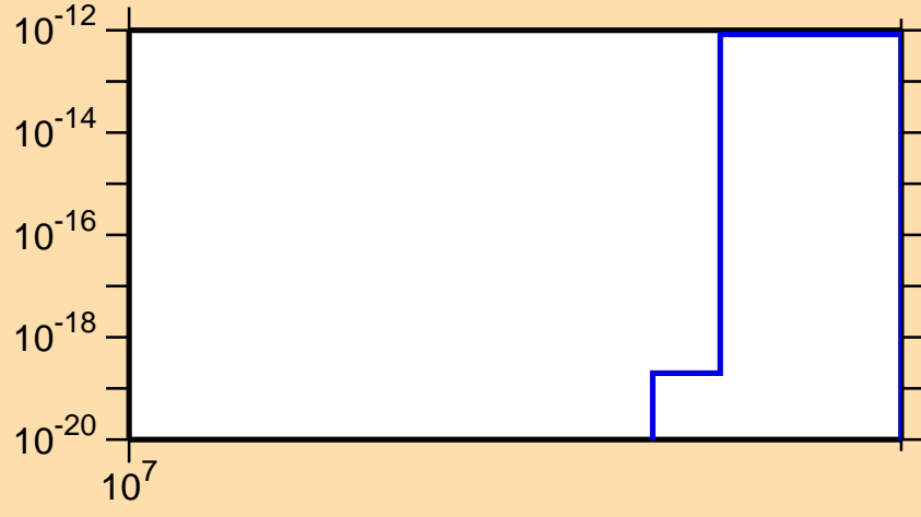
\sigma vs. E for ^{249}\text{Am} (mt 42)
