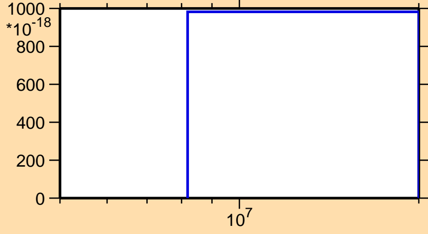
\sigma vs. E for ^{249}\text{Am}(n,\text{He}3)
