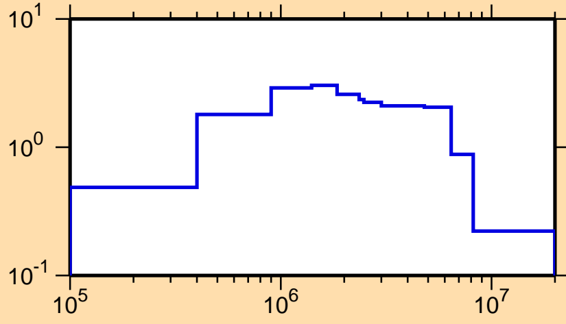
\sigma vs. E for ^{249}\text{Am}(n,\text{inel.})
