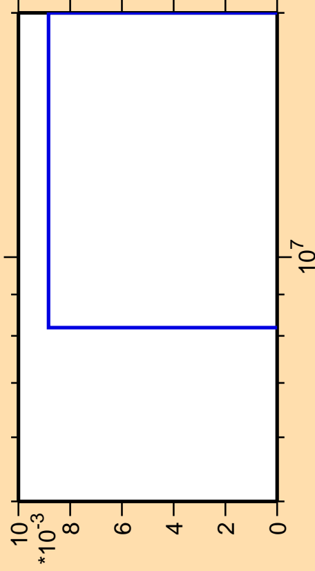
\Delta\sigma/\sigma vs. E for ^{249}\text{Am}(n,\text{He}3)
