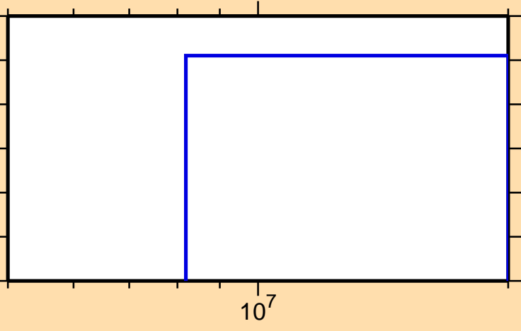
\sigma vs. E for ^{249}\text{Am}(n,2n\alpha)
