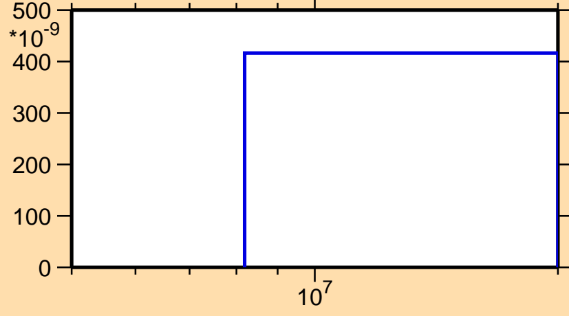
\sigma vs. E for ^{249}\text{Am}(n,nt)
