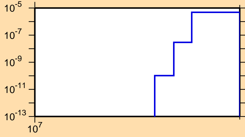
\sigma vs. E for ^{35}\text{Ar} (mt 45)
