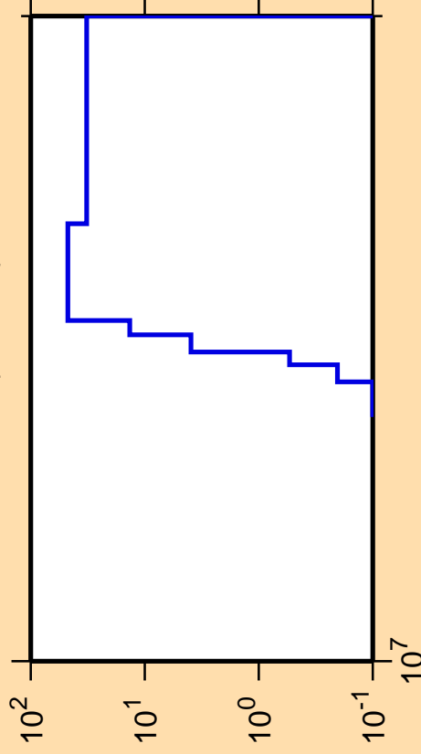
\Delta\sigma/\sigma vs. E for ^{35}\text{Ar}(\text{mt117})
