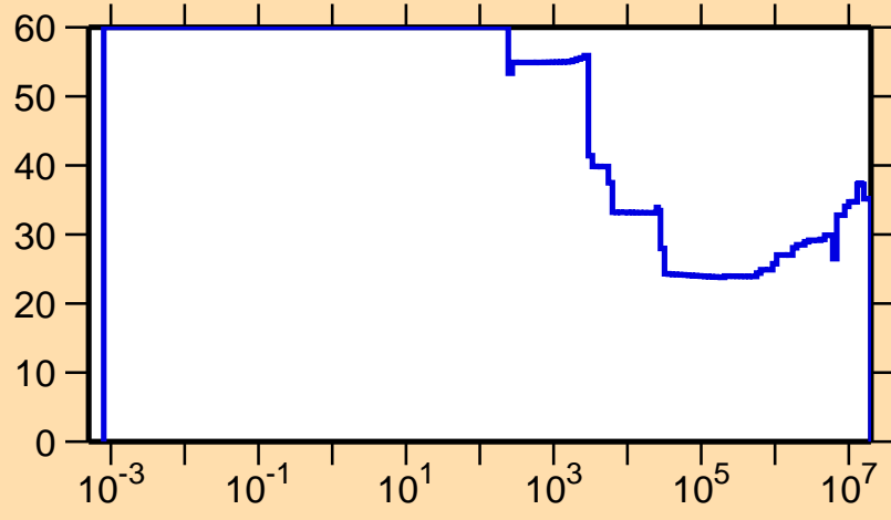
\Delta\sigma/\sigma vs. E for ^{35}\text{Ar}(n,\gamma)
