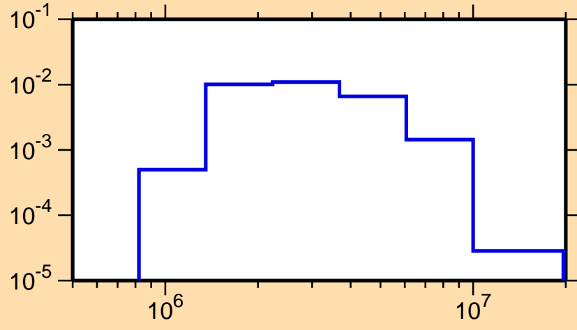
\sigma vs. E for ^{35}\text{Ar}(n,n_1)
