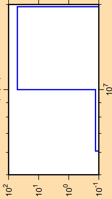
\Delta\sigma/\sigma vs. E for ^{35}\text{Ar}(n,pd)
