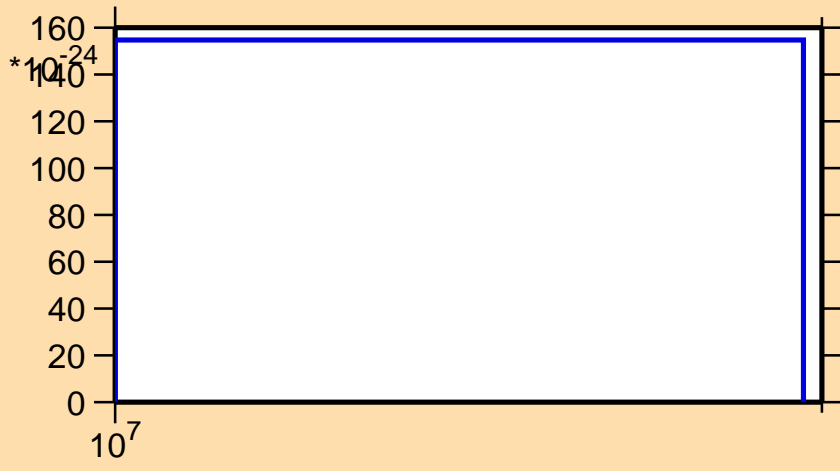
\sigma vs. E for ^{38}\text{Ar} (mt 45)
