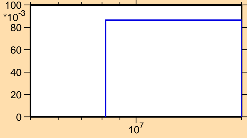
\sigma vs. E for ^{38}\text{Ar}(n,2n)
