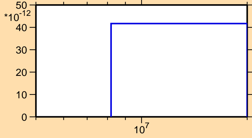
\sigma vs. E for ^{38}\text{Ar}(n,nd)
