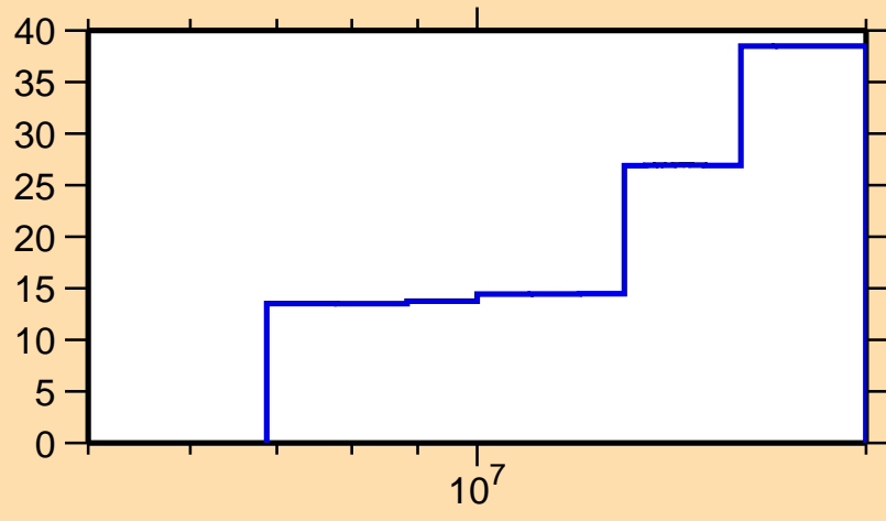
\Delta\sigma/\sigma vs. E for ^{40}\text{Ar}(n,ncont.)
