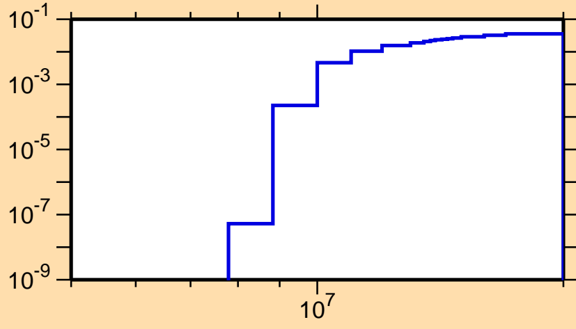
\sigma vs. E for ^{40}\text{Ar}(n,n\alpha)
