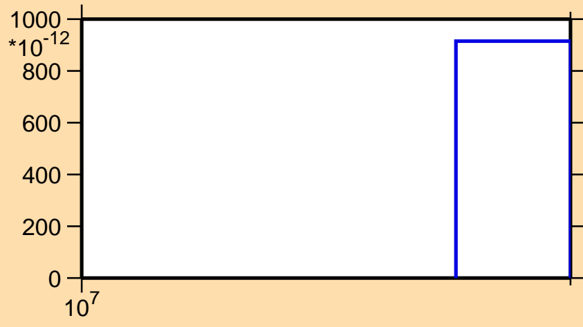
\sigma vs. E for ^{40}\text{Ar}(n,2n\alpha)
