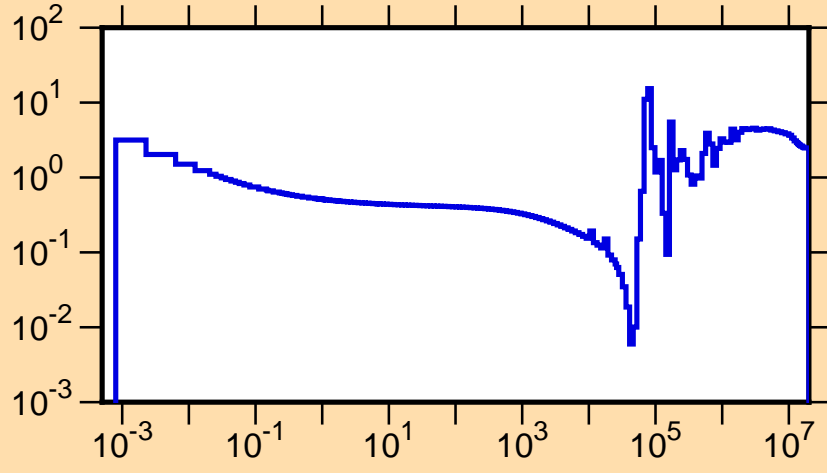
\sigma vs. E for ^{40}\text{Ar}(n,\text{tot.})
