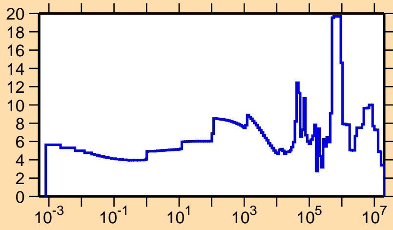
\Delta\sigma/\sigma vs. E for ^{40}\text{Ar}(n,\text{tot.})
