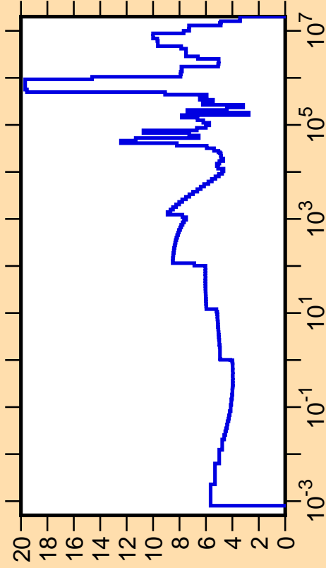
\Delta\sigma/\sigma vs. E for ^{40}\text{Ar}(n,\text{tot.})
