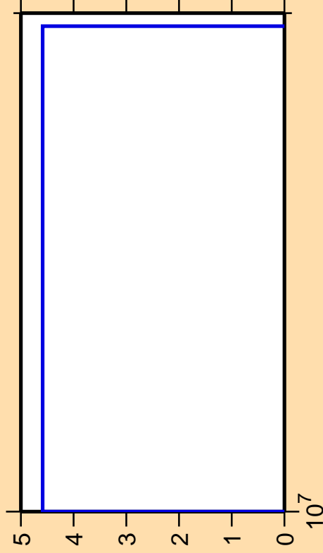
\Delta\sigma/\sigma vs. E for ^{40}\text{Ar}(n,nd)
