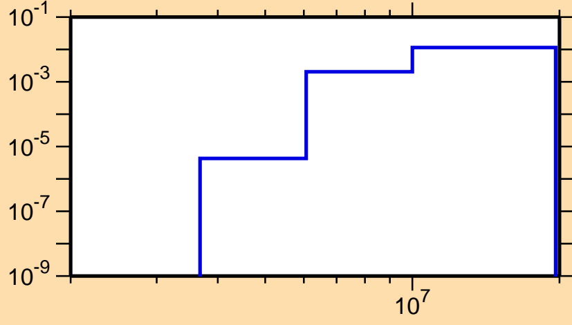
\sigma vs. E for ^{40}\text{Ar}(n,\alpha)
