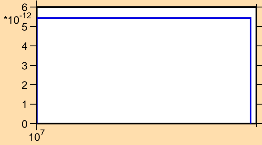
\sigma vs. E for ^{40}\text{Ar}(n,nd)
