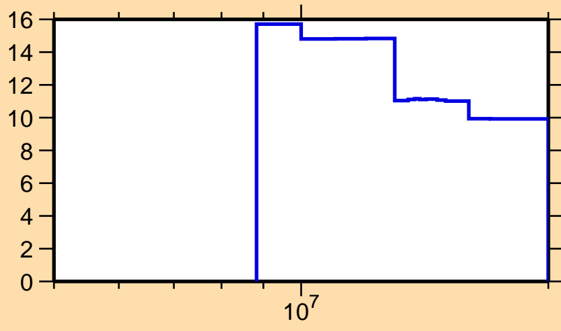
\Delta\sigma/\sigma vs. E for ^{42}\text{Ar}(n,el.)
