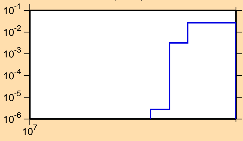
\sigma vs. E for ^{42}\text{Ar}(n,3n)
