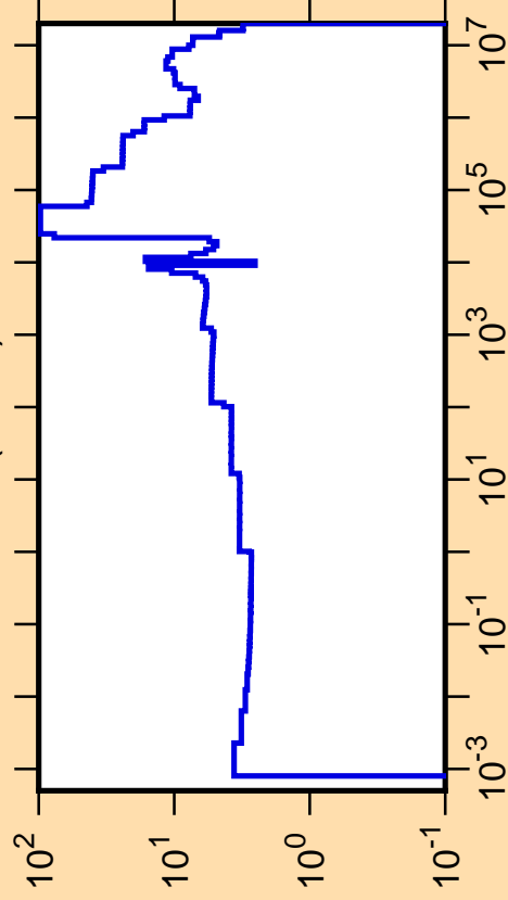
\Delta\sigma/\sigma vs. E for ^{42}\text{Ar}(n,\text{tot.})
