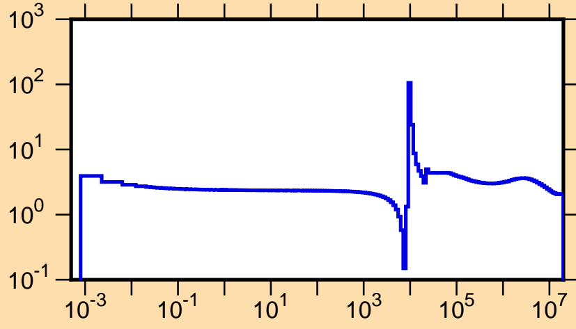
\sigma vs. E for ^{42}\text{Ar}(n,\text{tot.})
