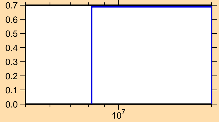
\sigma vs. E for ^{42}\text{Ar}(n,2n)
