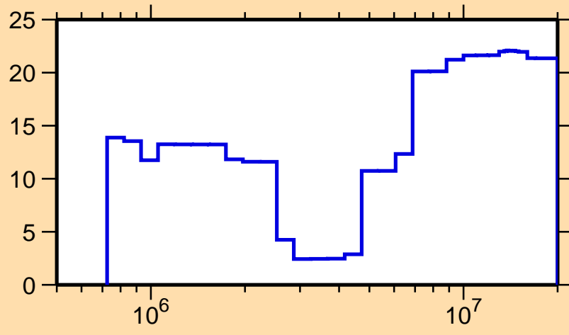
\Delta\sigma/\sigma vs. E for ^{43}\text{Ar}(n,n_1)
