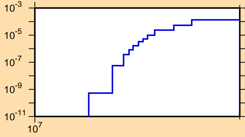
\sigma vs. E for ^{43}\text{Ar}(n,t)
