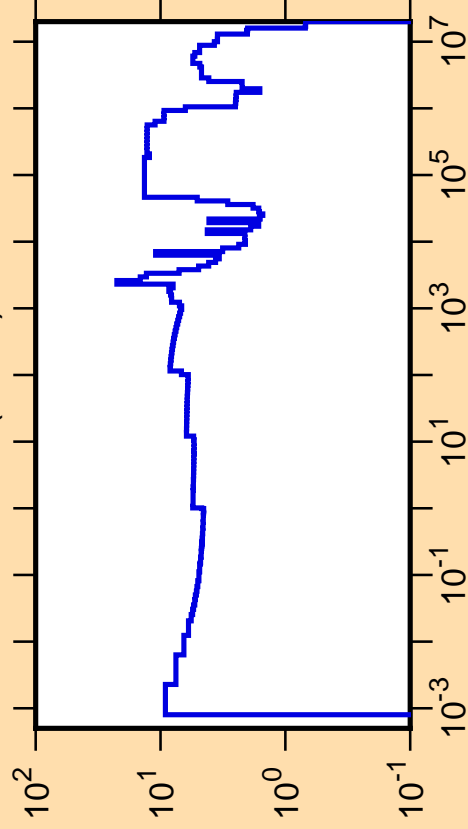
\Delta\sigma/\sigma vs. E for ^{43}\text{Ar}(n,\text{tot.})
