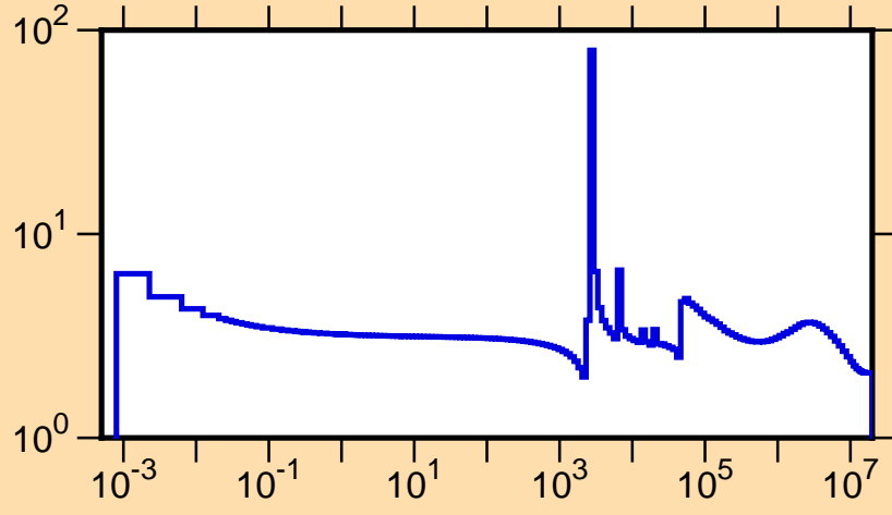
\sigma vs. E for ^{43}\text{Ar}(n,\text{tot.})
