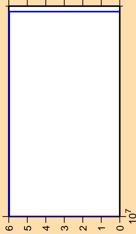
\Delta\sigma/\sigma vs. E for ^{43}\text{Ar}(n,2n\alpha)
