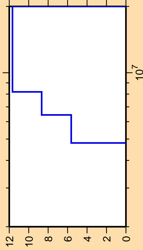
\Delta\sigma/\sigma vs. E for ^{43}\text{Ar}(n,\text{ncont.})
