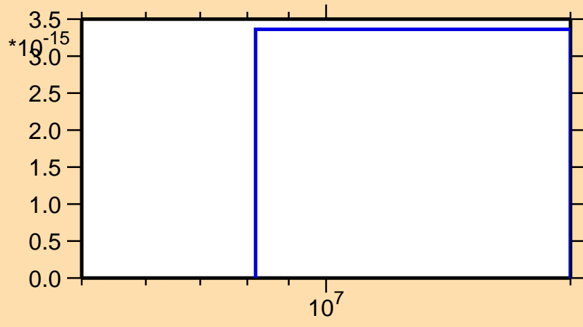
\sigma vs. E for ^{43}\text{Ar}(n,nt)
