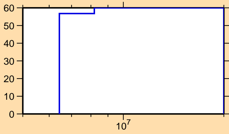
\Delta\sigma/\sigma vs. E for ^{43}\text{Ar}(n,\gamma)
