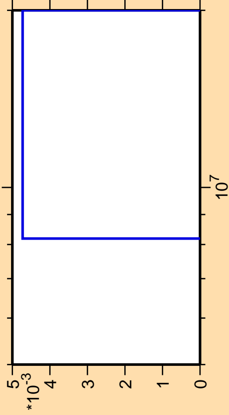
\Delta\sigma/\sigma vs. E for ^{43}\text{Ar}(n,nt)
