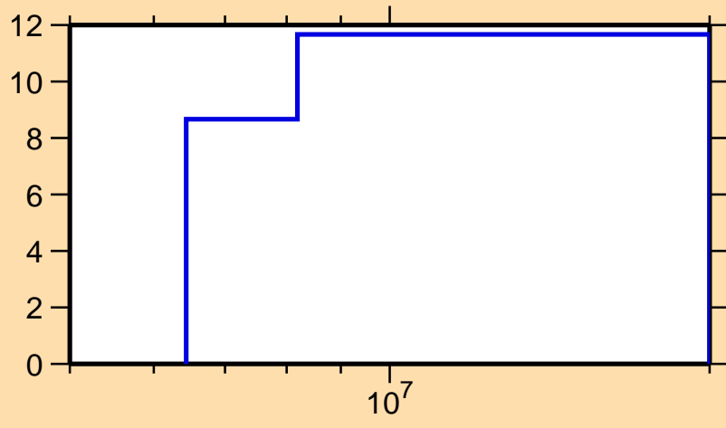
\Delta\sigma/\sigma vs. E for ^{43}\text{Ar}(n,ncont.)
