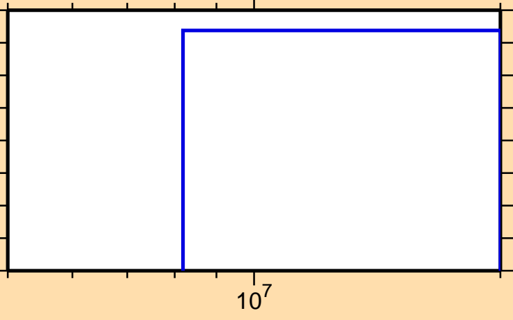
\sigma vs. E for ^{43}\text{Ar}(n,t)
