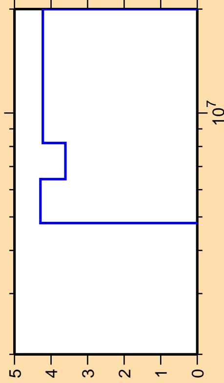
\Delta\sigma/\sigma vs. E for ^{43}\text{Ar}(n,2n)
