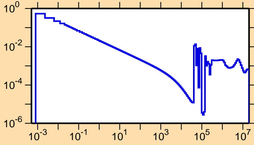
\sigma vs. E for ^{44}\text{Ar}(n,\gamma)
