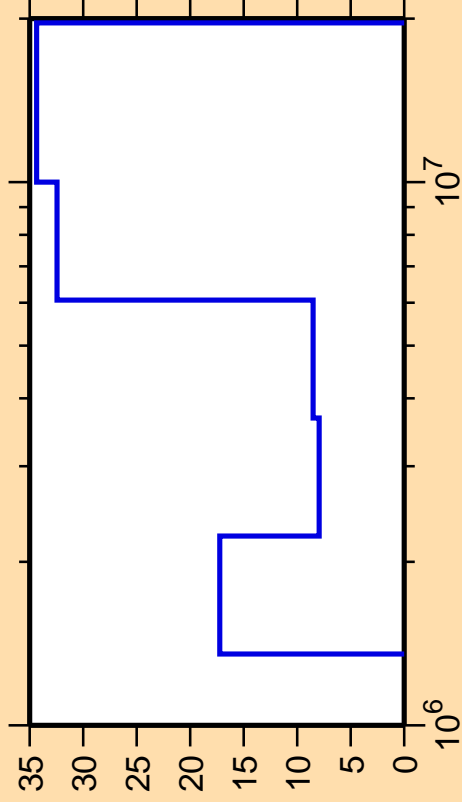
\Delta\sigma/\sigma vs. E for ^{44}\text{Ar}(n,n_3)
