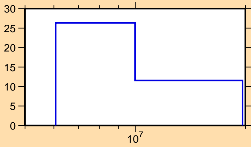
\Delta\sigma/\sigma vs. E for ^{44}\text{Ar}(n,2n)
