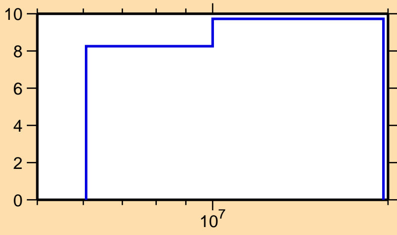
\Delta\sigma/\sigma vs. E for ^{44}\text{Ar}(n,\text{nonel.})
