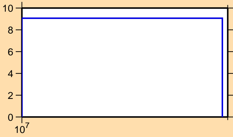
\Delta\sigma/\sigma vs. E for ^{44}\text{Ar}(n,el.)
