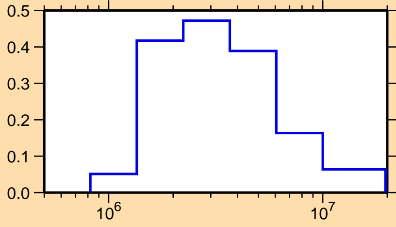
\sigma vs. E for ^{44}\text{Ar}(n,n_2)
