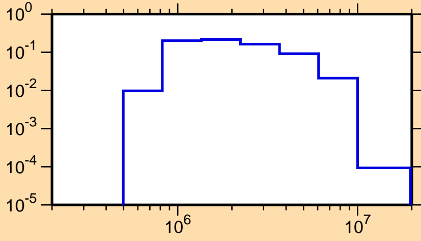
\sigma vs. E for ^{44}\text{Ar}(n,n_1)
