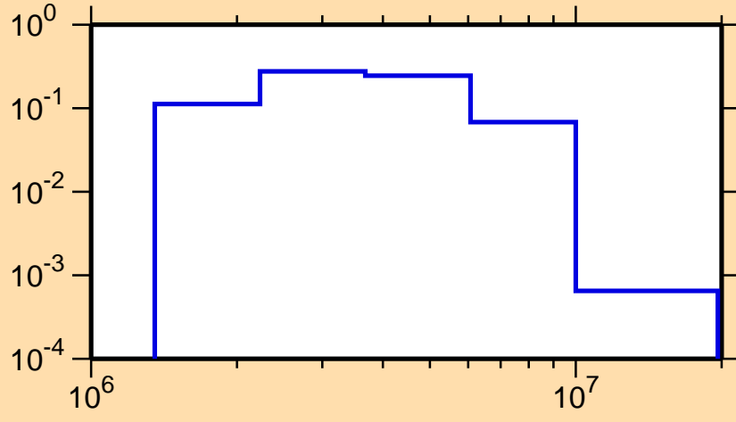
\sigma vs. E for ^{44}\text{Ar}(n,n_3)
