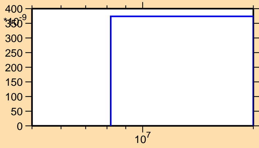
\sigma vs. E for ^{44}\text{Ar}(n,\alpha)
