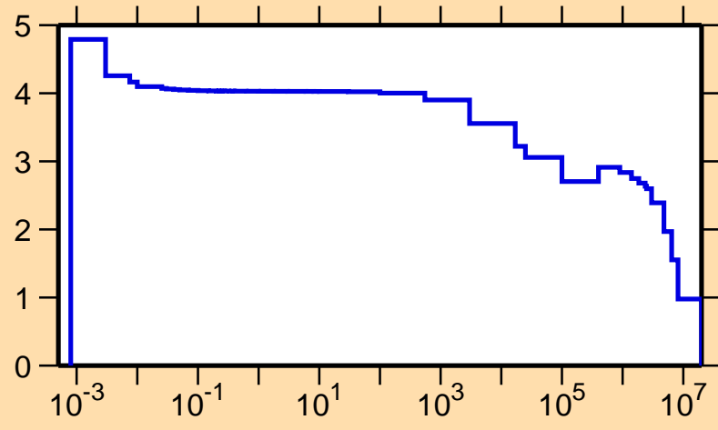
\sigma vs. E for ^{44}\text{Ar}(n,\text{el.})
