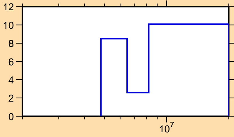
\Delta\sigma/\sigma vs. E for ^{44}\text{Ar}(n,inel.)
