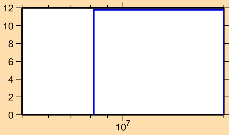
\Delta\sigma/\sigma vs. E for ^{44}\text{Ar}(n,ncont.)
