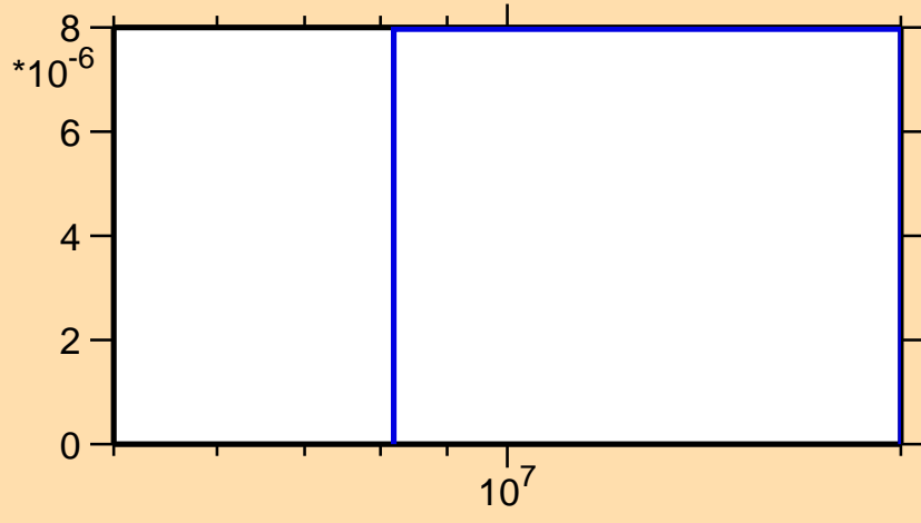
\sigma vs. E for ^{44}\text{Ar}(n,d)
