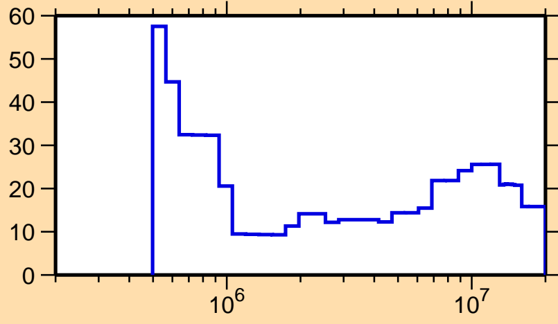
\Delta\sigma/\sigma vs. E for ^{45}\text{Ar}(n,\text{el.})
