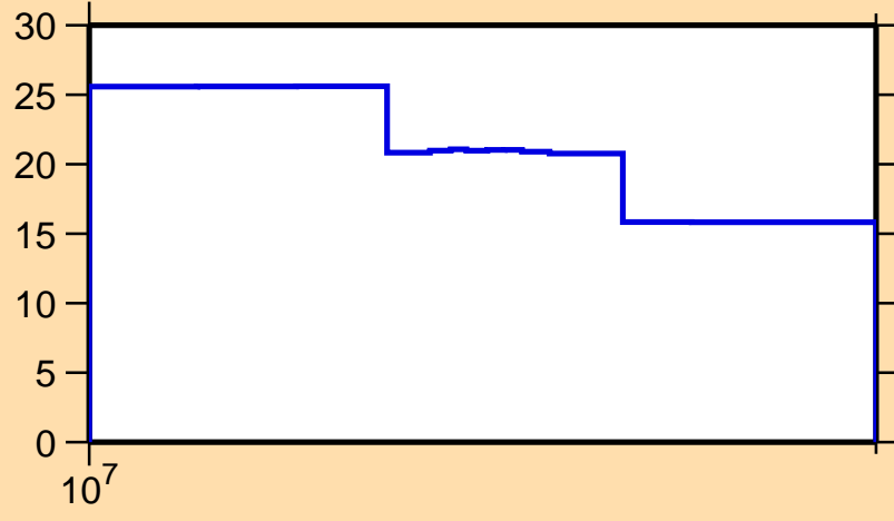
\Delta\sigma/\sigma vs. E for ^{45}\text{Ar}(n,\text{el.})
