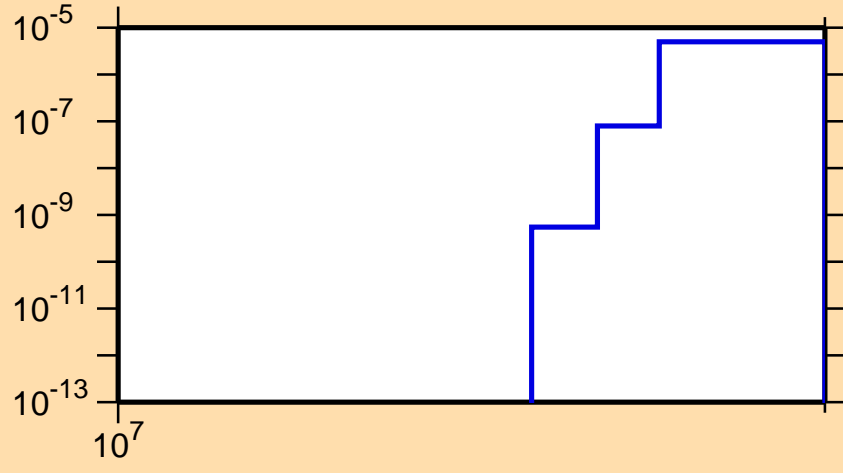
\sigma vs. E for ^{45}\text{Ar}(n,n\alpha)
