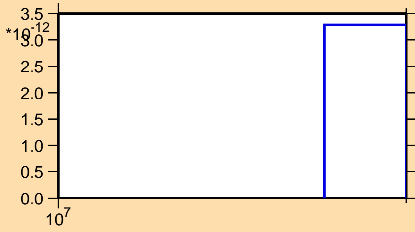
\sigma vs. E for ^{45}\text{Ar}(n,\text{nd})
