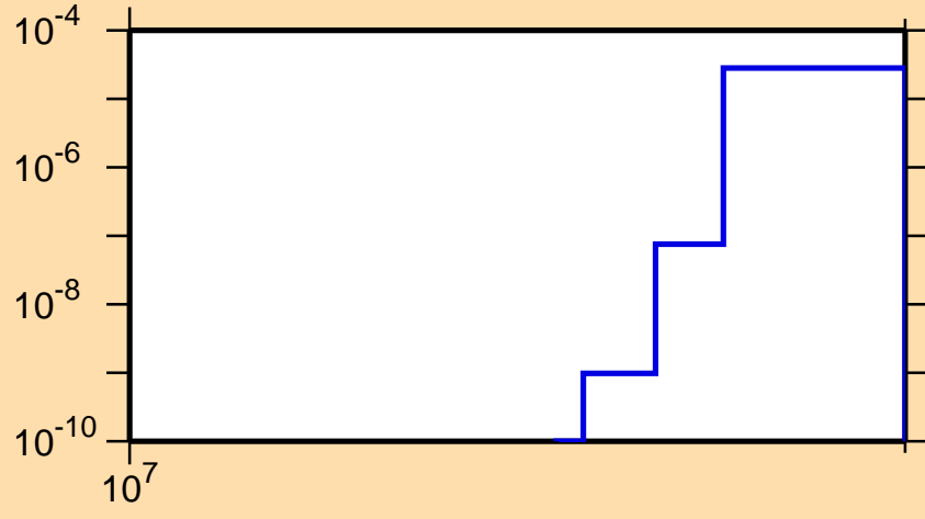
\sigma vs. E for ^{45}\text{Ar}(n,d)
