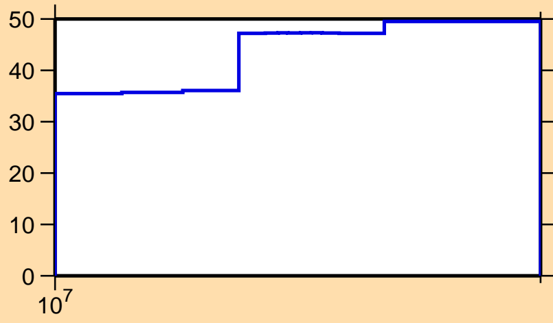
\Delta\sigma/\sigma vs. E for ^{45}\text{Ar}(n,n\text{cont.})
