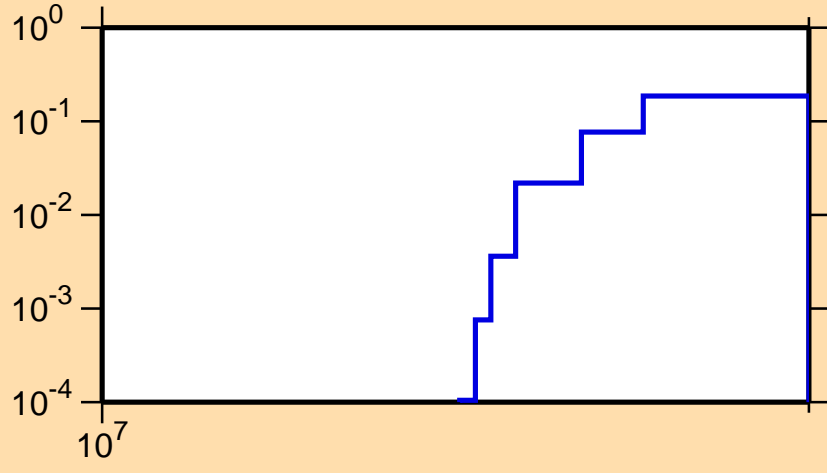
\sigma vs. E for ^{45}\text{Ar}(n,3n)
