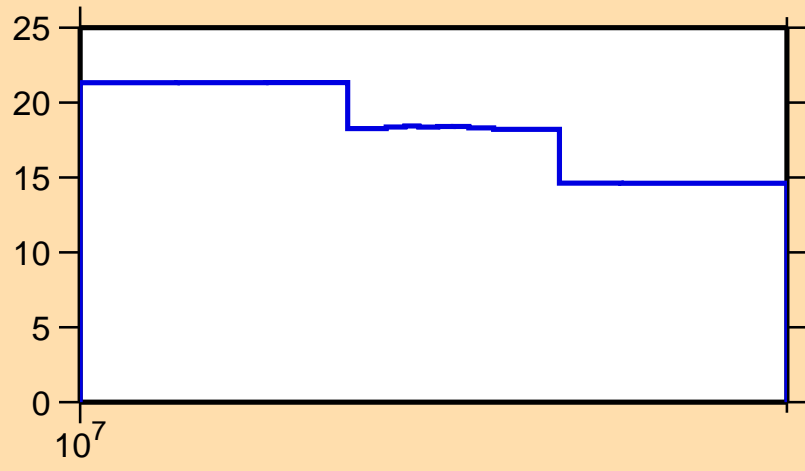
\Delta\sigma/\sigma vs. E for ^{45}\text{Ar}(n,\text{tot.})
