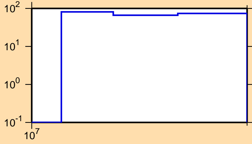
\Delta\sigma/\sigma vs. E for ^{45}\text{Ar}(n,p)
