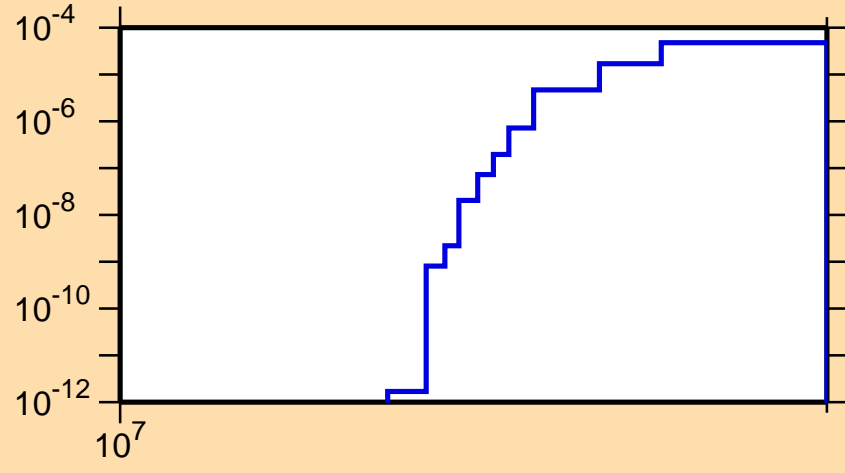
\sigma vs. E for ^{45}\text{Ar}(n,t)
