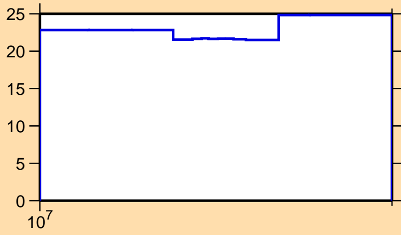
\Delta\sigma/\sigma vs. E for ^{45}\text{Ar}(n,2n)
