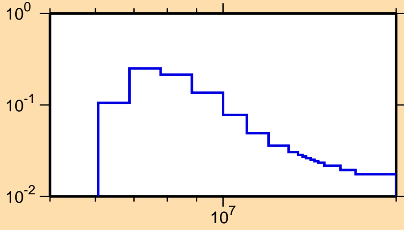
\sigma vs. E for ^{45}\text{Ar}(n,n\text{cont.})
