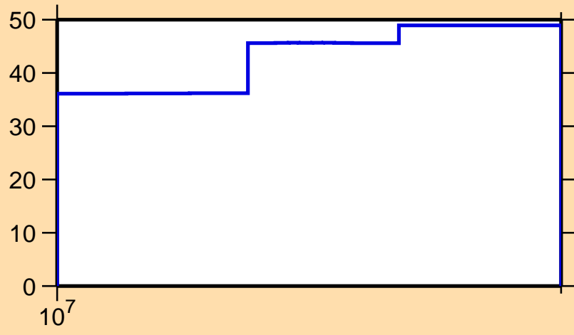
\Delta\sigma/\sigma vs. E for ^{45}\text{Ar}(n,\text{inel.})
