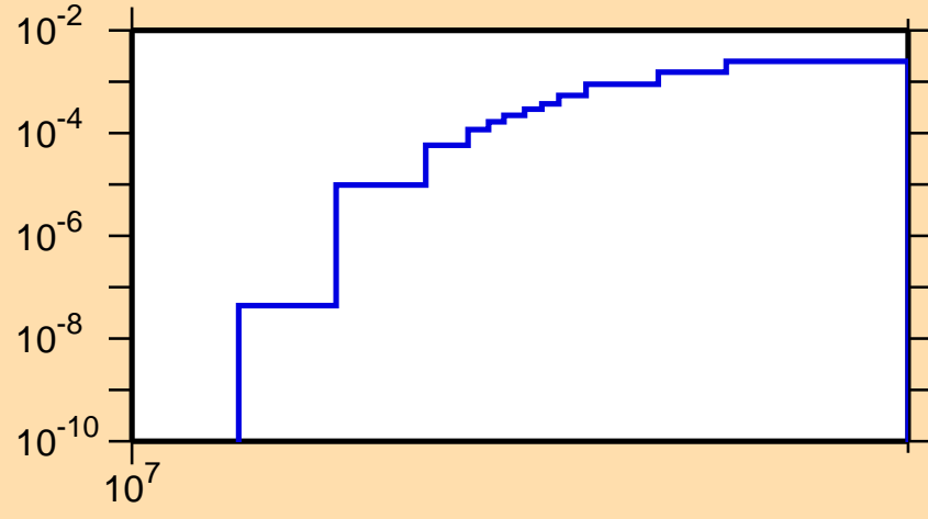
\sigma vs. E for ^{45}\text{Ar}(n,p)
