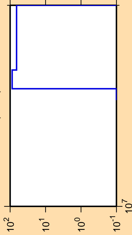
\Delta\sigma/\sigma vs. E for ^{45}\text{Ar}(n,n\alpha)
