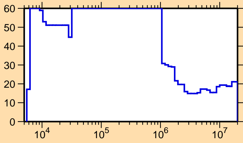
\Delta\sigma/\sigma vs. E for ^{45}\text{Ar}(n,\text{nonel.})
