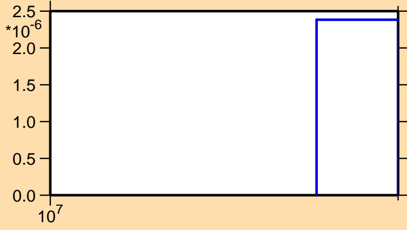
\sigma vs. E for ^{45}\text{Ar}(n,np)
