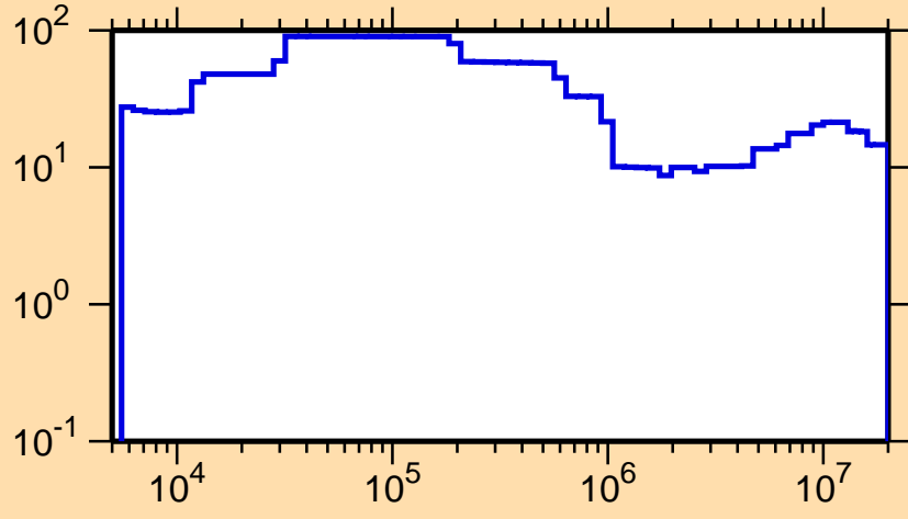
\Delta\sigma/\sigma vs. E for ^{45}\text{Ar}(n,\text{tot.})
