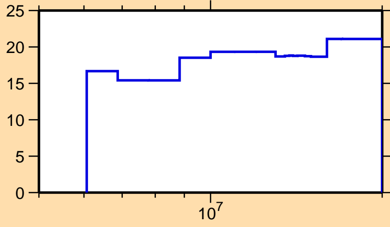
\Delta\sigma/\sigma vs. E for ^{45}\text{Ar}(n,\text{nonel.})
