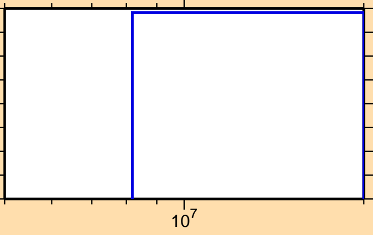
\sigma vs. E for ^{47}\text{Ar}(n,n\alpha)
