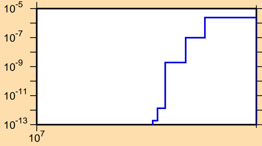
\sigma vs. E for ^{67}\text{As}(n,nd)
