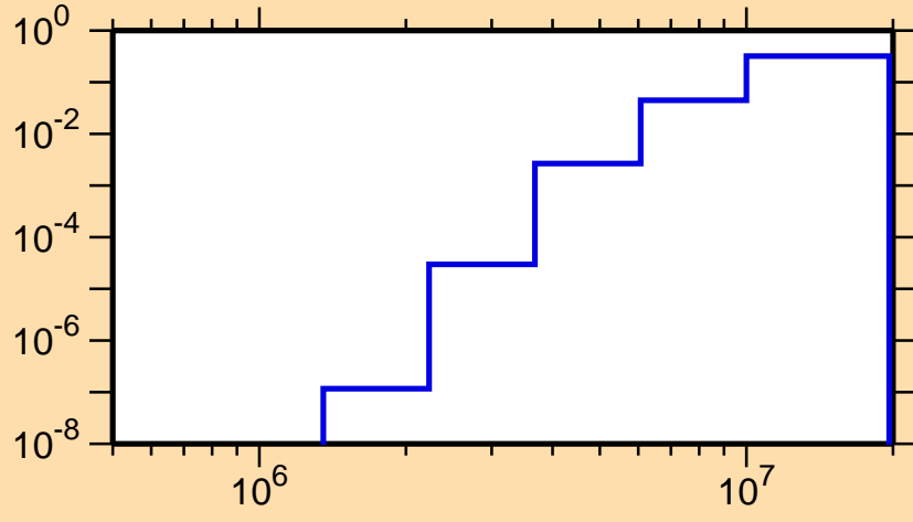
\sigma vs. E for ^{67}\text{As}(n,p\alpha)
