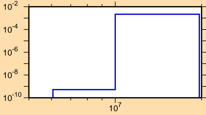
\sigma vs. E for ^{67}\text{As}(n,pd)
