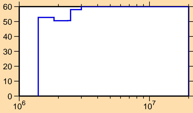
\Delta\sigma/\sigma vs. E for ^{67}\text{As}(n,n_1)
