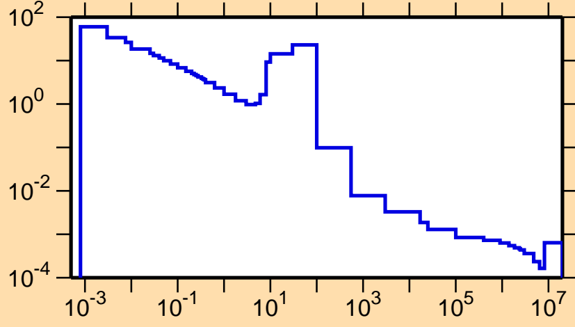
\sigma vs. E for ^{67}\text{As}(n,\gamma)
