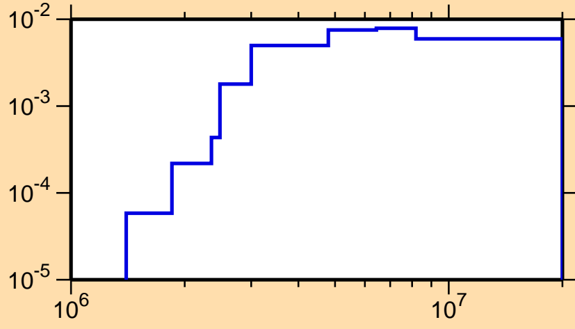
\sigma vs. E for ^{67}\text{As}(n,n\text{cont.})
