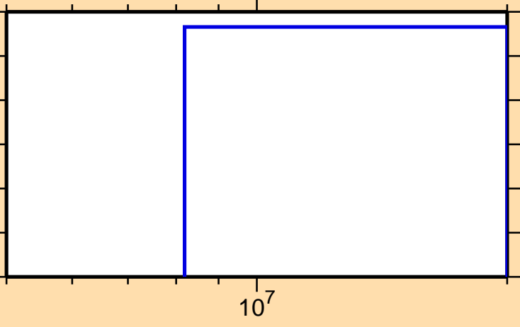
\sigma vs. E for ^{67}\text{As}(n,2np)
