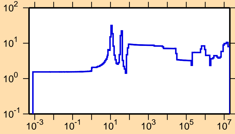
\Delta\sigma/\sigma vs. E for ^{68}\text{As}(n,el.)
