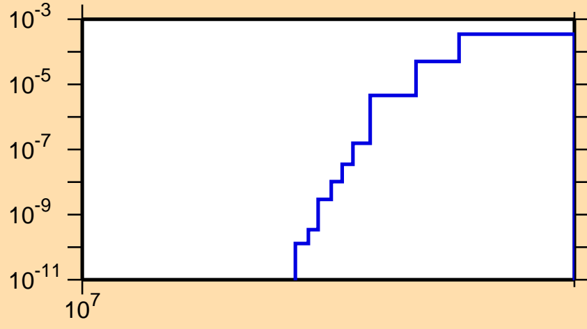
\sigma vs. E for ^{68}\text{As}(n,pt)
