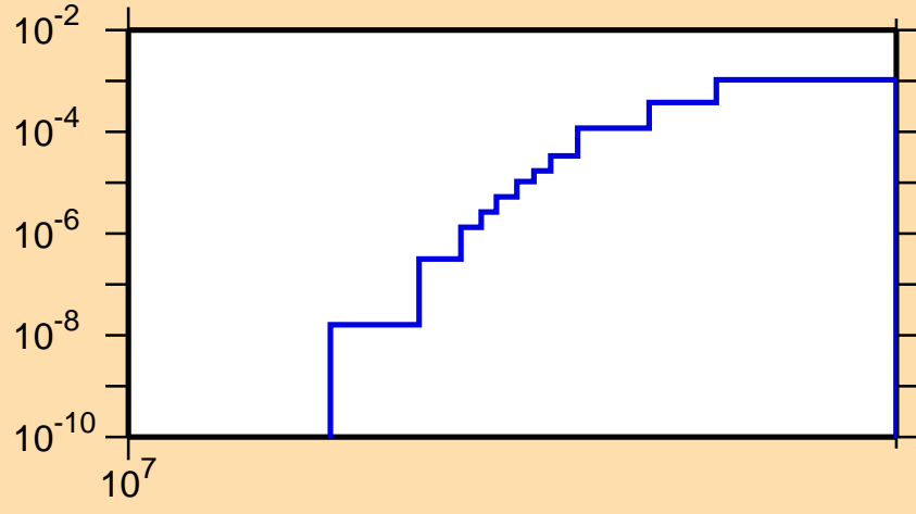
\sigma vs. E for ^{70}\text{As}(n,nd)
