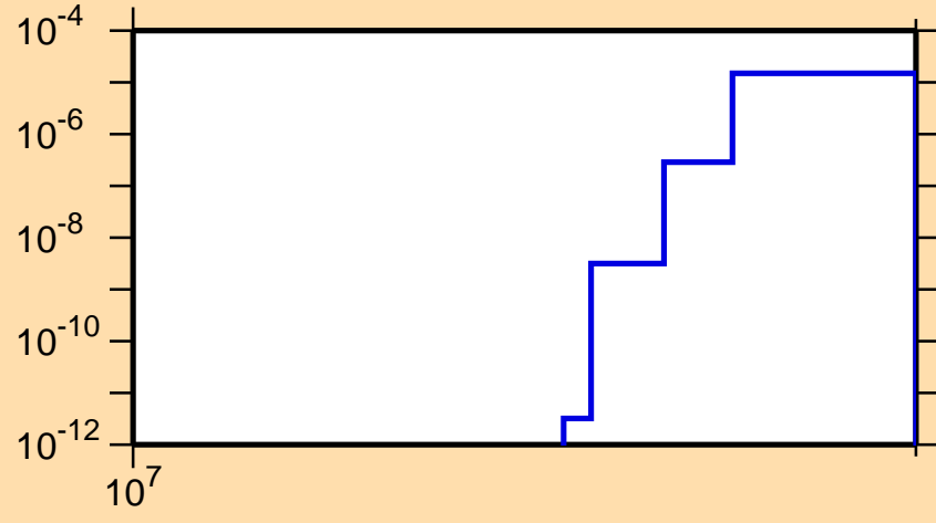
\sigma vs. E for ^{70}\text{As}(n,pt)
