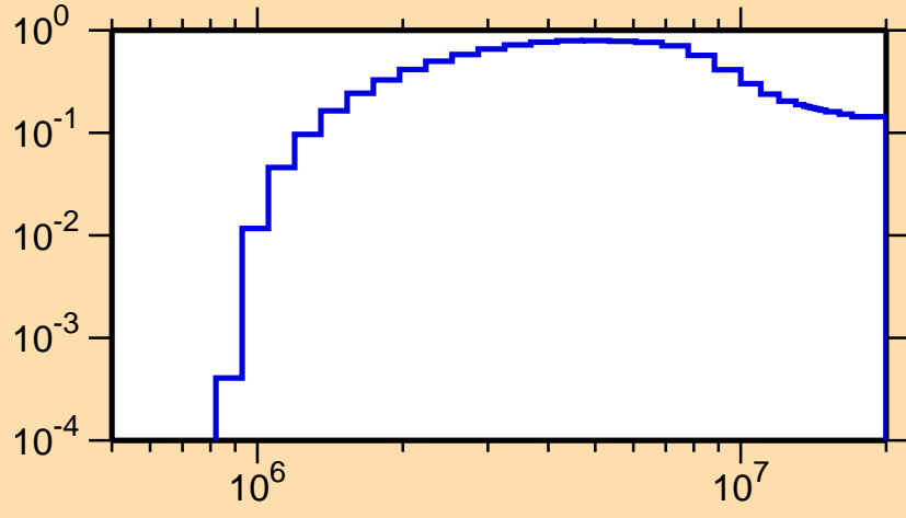
\sigma vs. E for ^{70}\text{As}(n,n\text{cont.})
