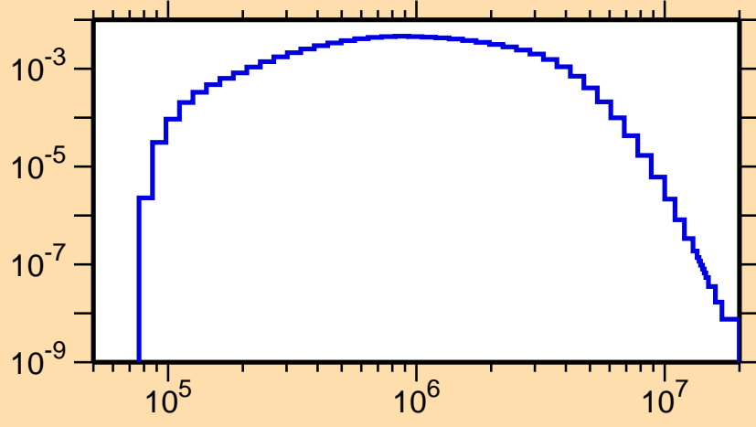
\sigma vs. E for ^{70}\text{As}(n,n_2)
