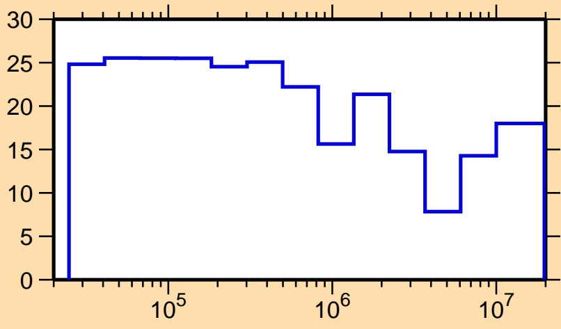
\Delta\sigma/\sigma vs. E for ^{70}\text{As}(n,\text{el.})
