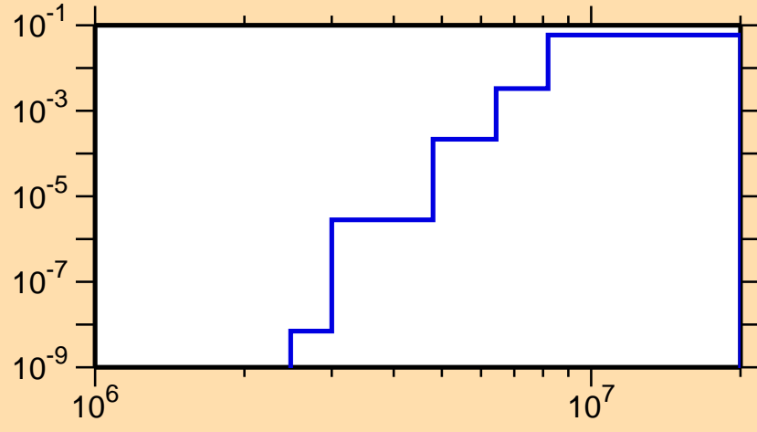
\sigma vs. E for ^{70}\text{As}(n,p\alpha)
