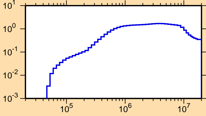
\sigma vs. E for ^{72}\text{As}(n,\text{inel.})
