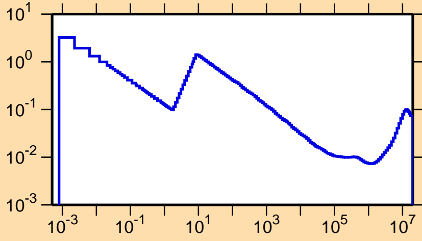
\sigma vs. E for ^{72}\text{As}(n,\alpha)
