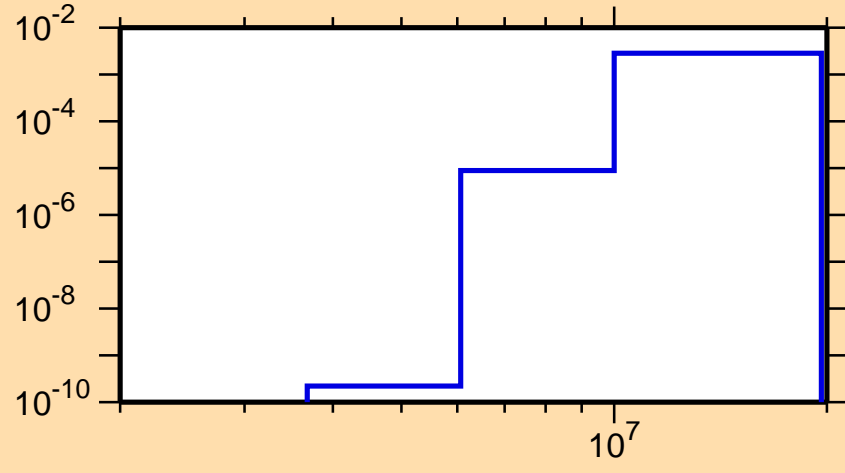
\sigma vs. E for ^{72}\text{As}(n,p\alpha)
