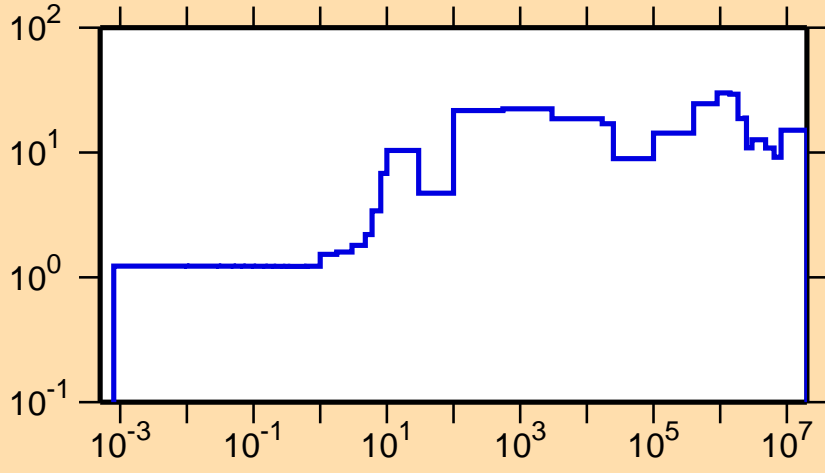
\Delta\sigma/\sigma vs. E for ^{72}\text{As}(n,el.)
