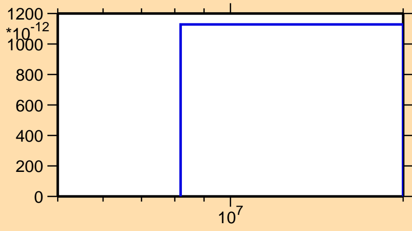
\sigma vs. E for ^{72}\text{As}(n,pt)
