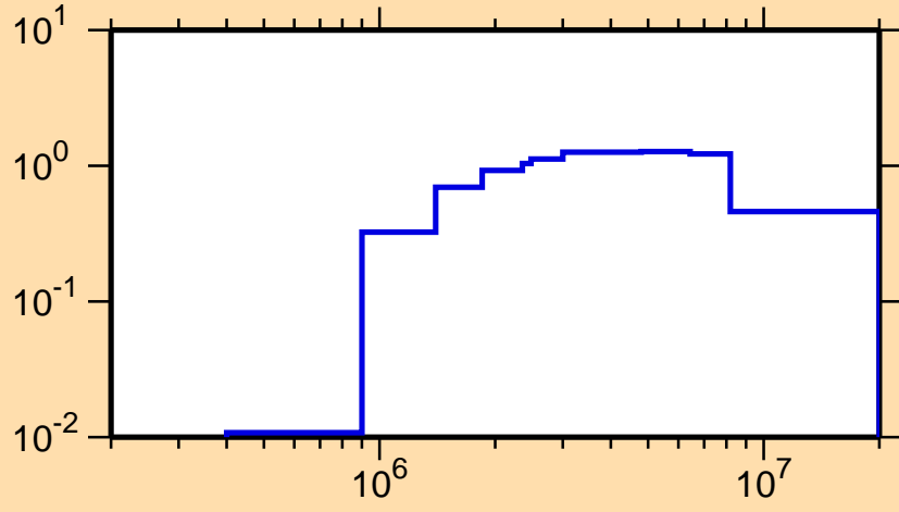
\sigma vs. E for ^{72}\text{As}(n,n\text{cont.})
