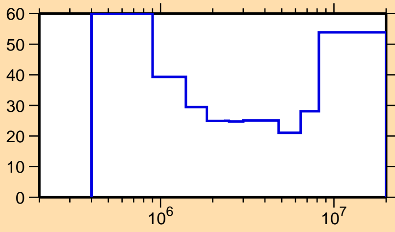
\Delta\sigma/\sigma vs. E for ^{72}\text{As}(n,ncont.)
