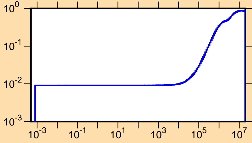
\mu vs. E for ^{74}\text{As}(\text{mt251})
