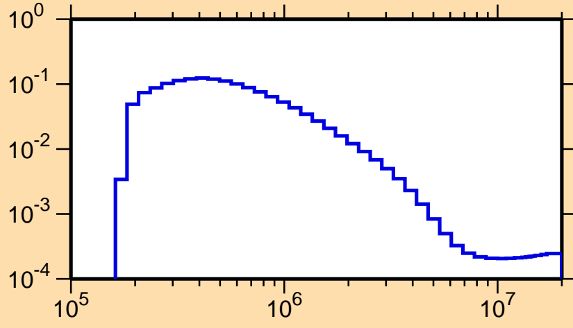
\sigma vs. E for ^{74}\text{As}(n,n_1)
