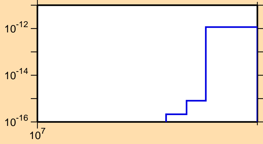
\sigma vs. E for ^{74}\text{As}(n,pt)
