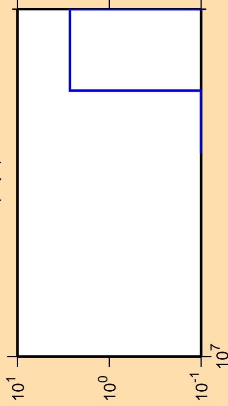
\Delta\sigma/\sigma vs. E for ^{74}\text{As}(n,pt)
