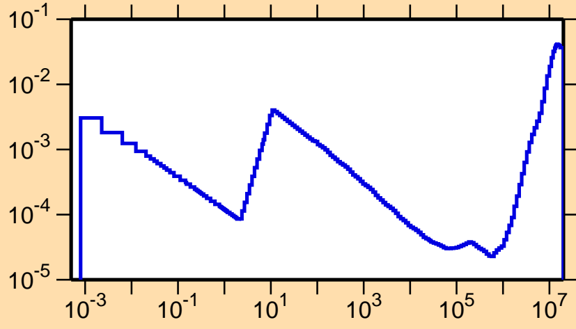
\sigma vs. E for ^{74}\text{As}(n,\alpha)
