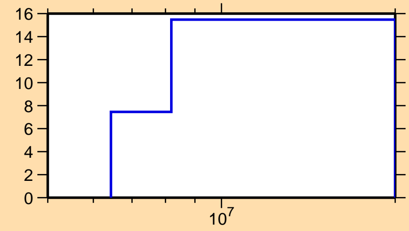
\Delta\sigma/\sigma vs. E for ^{74}\text{As}(n,\text{incl.})
