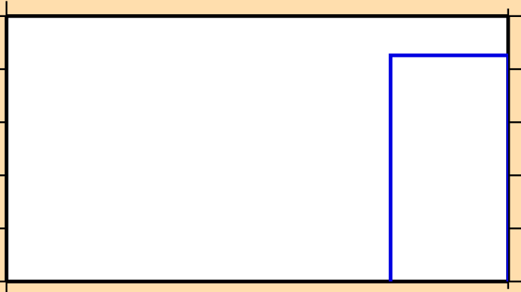
\sigma vs. E for ^{75}\text{As}(n,\text{pt})
