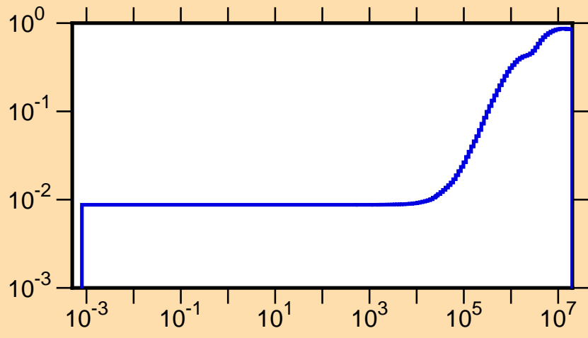
\mu vs. E for ^{77}\text{As}(\text{mt251})
