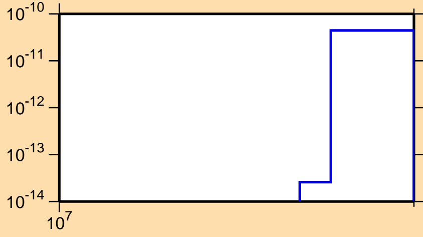
\sigma vs. E for ^{77}\text{As}(n,\text{He3})
