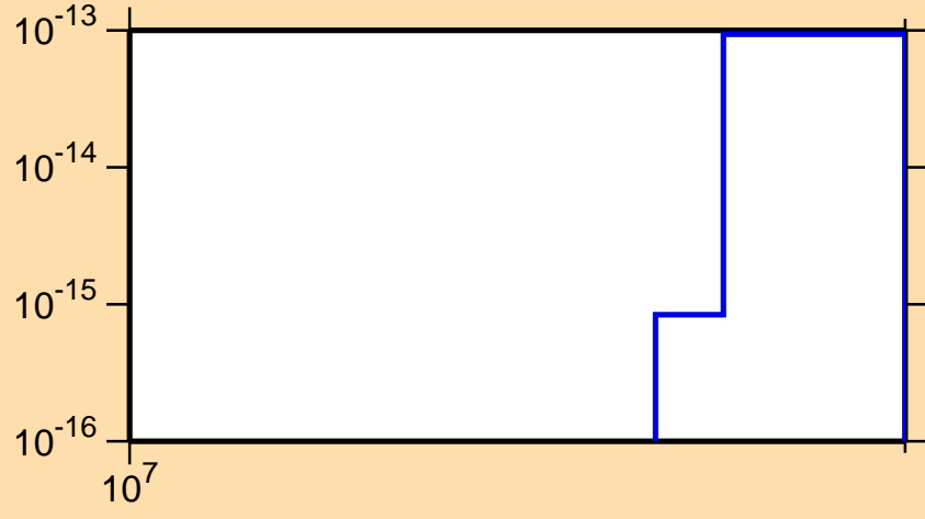
\sigma vs. E for ^{77}\text{As}(n,2n\alpha)
