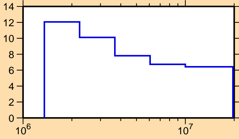
\Delta\sigma/\sigma vs. E for ^{77}\text{As}(n,n\text{oncl.})
