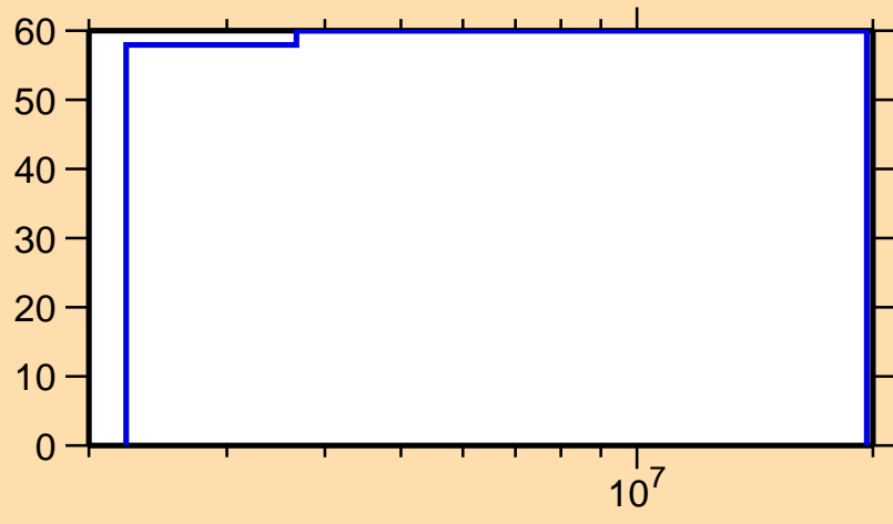
\Delta\sigma/\sigma vs. E for ^{77}\text{As}(n,\gamma)
