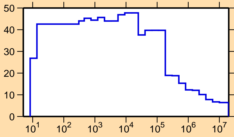
\Delta\sigma/\sigma vs. E for ^{77}\text{As}(n,\text{nonel.})
