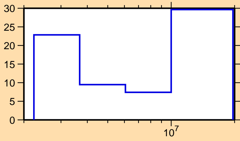
\Delta\sigma/\sigma vs. E for ^{77}\text{As}(n,ncont.)
