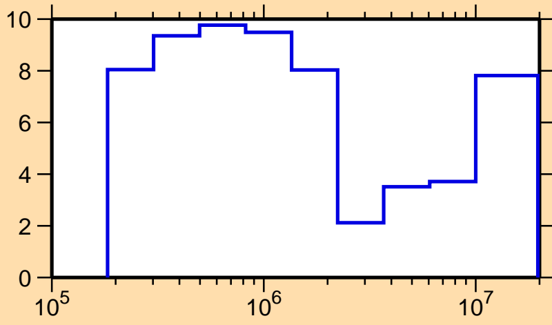
\Delta\sigma/\sigma vs. E for ^{77}\text{As}(n,\text{tot.})
