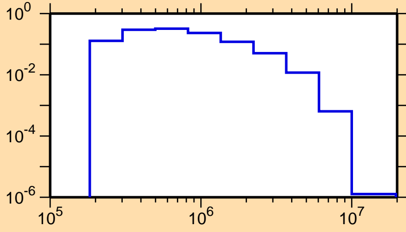
\sigma vs. E for ^{77}\text{As}(n,n_1)
