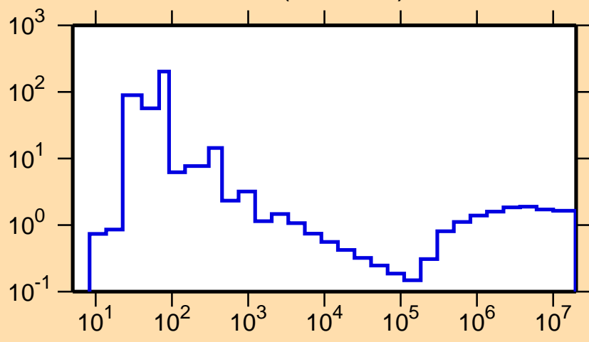
\sigma vs. E for ^{77}\text{As}(n,\text{nonel.})
