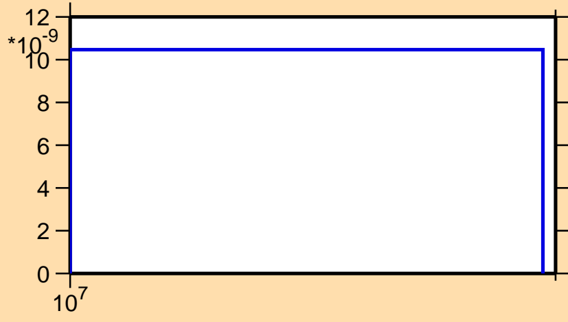
\sigma vs. E for ^{77}\text{As}(n,nd)
