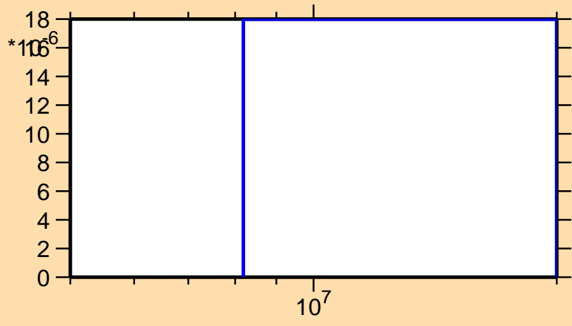
\sigma vs. E for ^{77}\text{As}(n,t)
