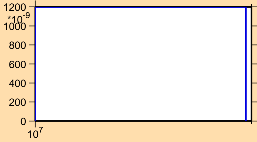
\sigma vs. E for ^{78}\text{As}(n,nd)
