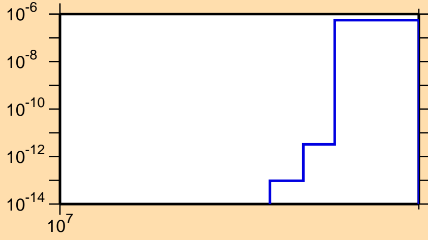
\sigma vs. E for ^{79}\text{As}(n,nd)
