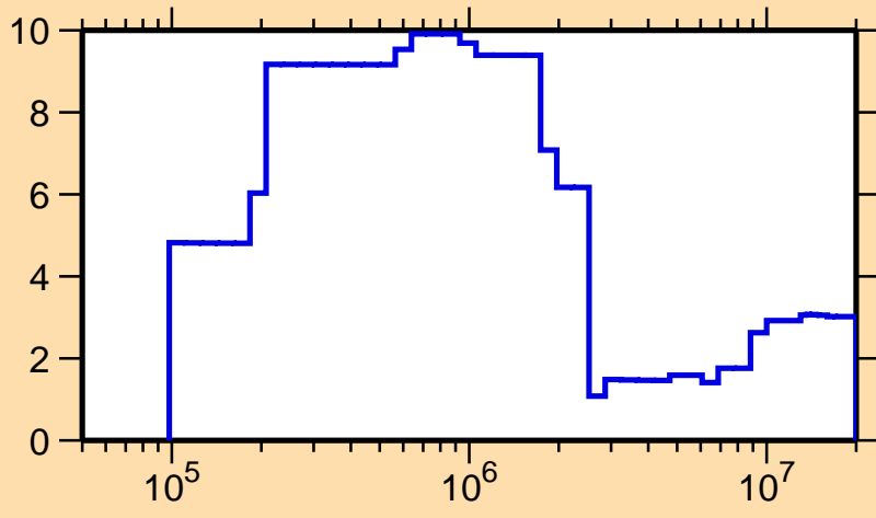
\Delta\sigma/\sigma vs. E for ^{79}\text{As}(n,\text{tot.})
