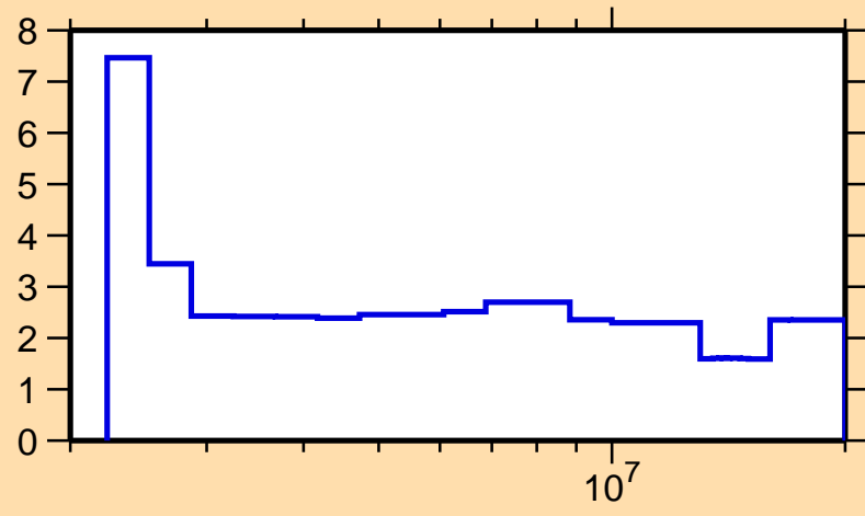
\Delta\sigma/\sigma vs. E for ^{79}\text{As}(n,n\text{oncl.})
