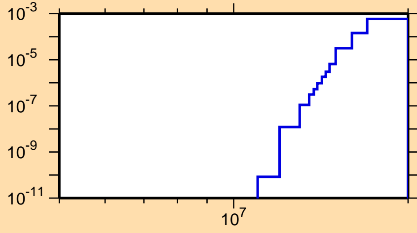
\sigma vs. E for ^{79}\text{As}(n,n\alpha)
