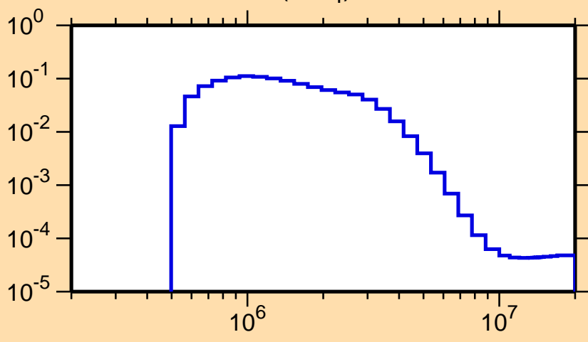
\sigma vs. E for ^{79}\text{As}(n,n_4)
