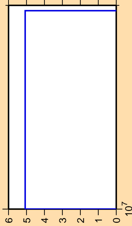
\Delta\sigma/\sigma vs. E for ^{79}\text{As}(n,2np)
