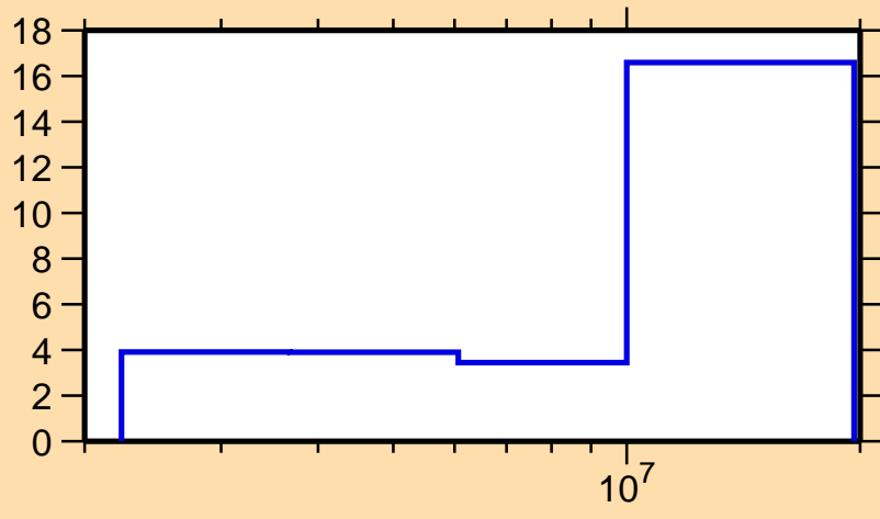
\Delta\sigma/\sigma vs. E for ^{79}\text{As}(n,ncont.)
