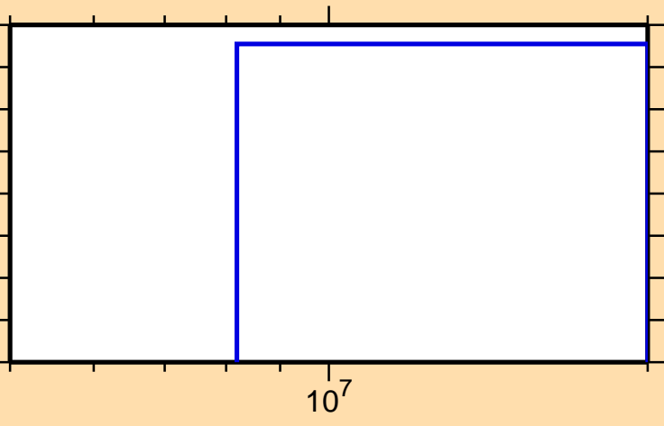
\sigma vs. E for ^{79}\text{As}(n,n\alpha)
