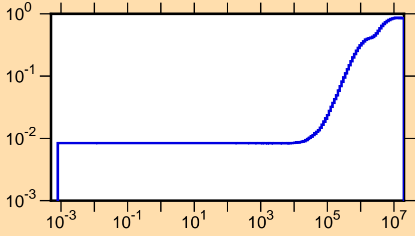
\mu vs. E for ^{80}\text{As}(\text{mt251})
