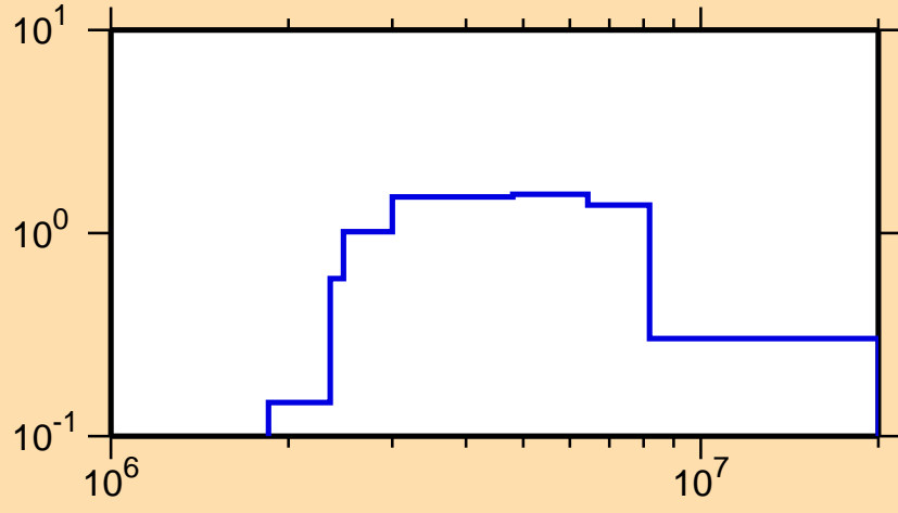
\sigma vs. E for ^{80}\text{As}(n,n\text{cont.})
