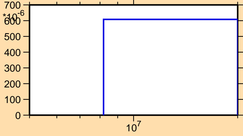
\sigma vs. E for ^{80}\text{As}(n,d)
