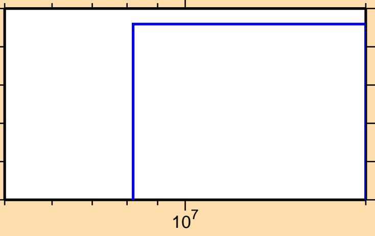
\sigma vs. E for ^{80}\text{As}(n,2np)
