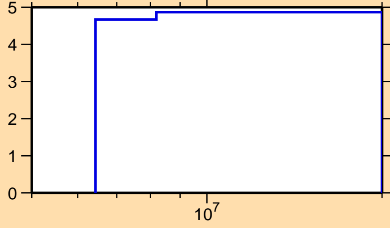
\Delta\sigma/\sigma vs. E for ^{80}\text{As}(n,\text{tot.})
