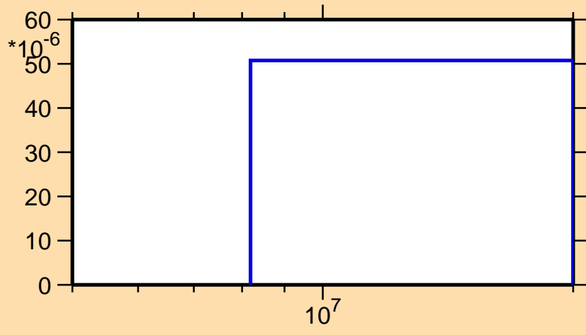
\sigma vs. E for ^{80}\text{As}(n,t)
