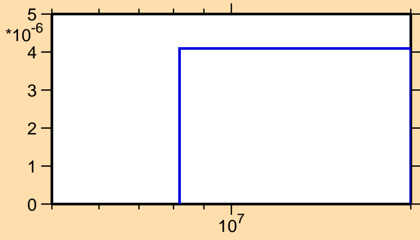
\sigma vs. E for ^{80}\text{As}(n,n\alpha)
