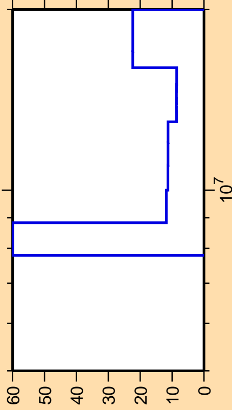
\Delta\sigma/\sigma vs. E for ^{81}\text{As}(n,2n)
