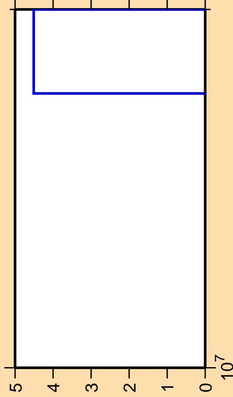
\Delta\sigma/\sigma vs. E for ^{81}\text{As}(n,2np)
